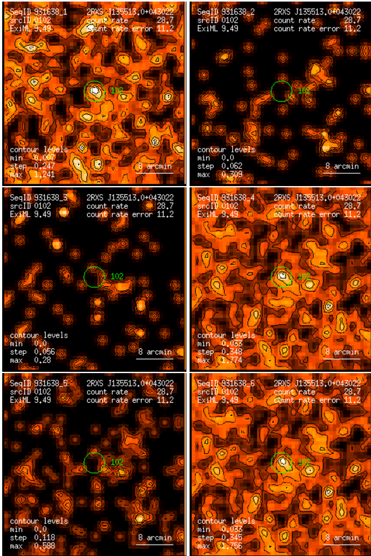
Figure 102: RASS 931638: detection 0102: band rate images, Gaussian filter: (1) PSPC channels 11 – 41, (2) 52 – 90, (3) 91 – 201, (4) 11 – 235, (5) 52 – 201, (6) 11 – 201. Broad band rates in counts/ks. Band rate contour levels in counts/ks/arcmin 2 .
