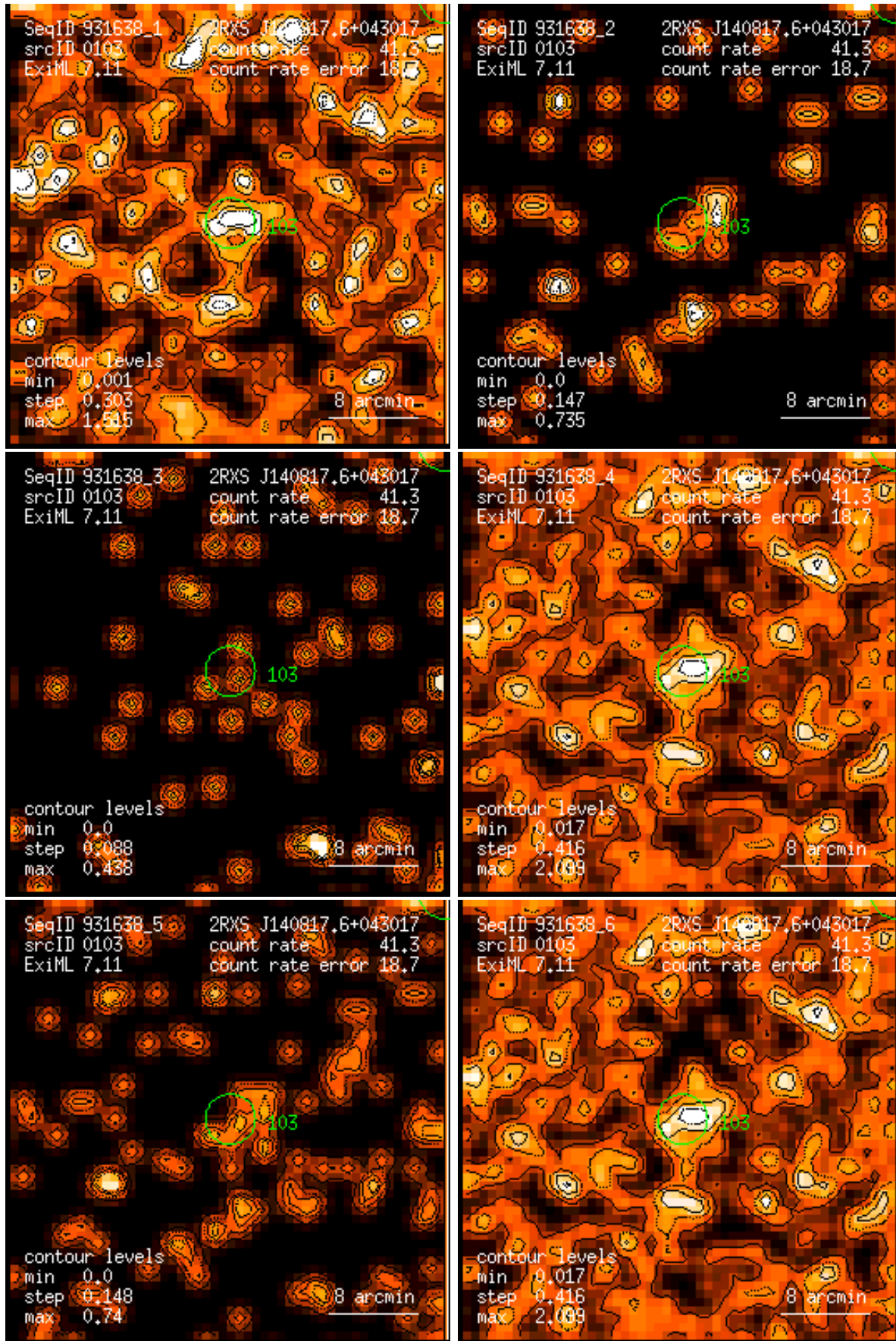
Figure 103: RASS 931638: detection 0103: band rate images, Gaussian filter: (1) PSPC channels 11 – 41, (2) 52 – 90, (3) 91 – 201, (4) 11 – 235, (5) 52 – 201, (6) 11 – 201. Broad band rates in counts/ks. Band rate contour levels in counts/ks/arcmin 2 .
