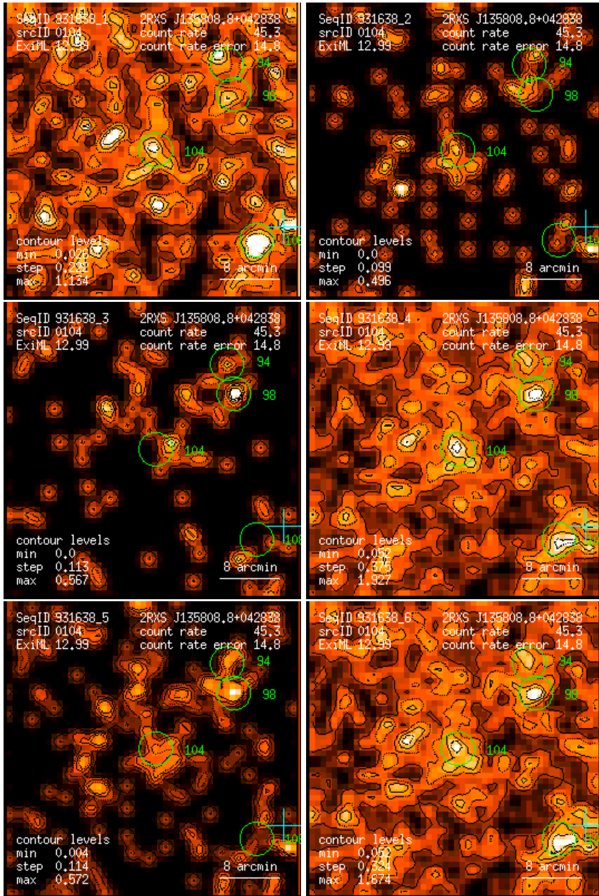
Figure 104: RASS 931638: detection 0104: band rate images, Gaussian filter: (1) PSPC channels 11 – 41, (2) 52 – 90, (3) 91 – 201, (4) 11 – 235, (5) 52 – 201, (6) 11 – 201. Broad band rates in counts/ks. Band rate contour levels in counts/ks/arcmin 2 .
