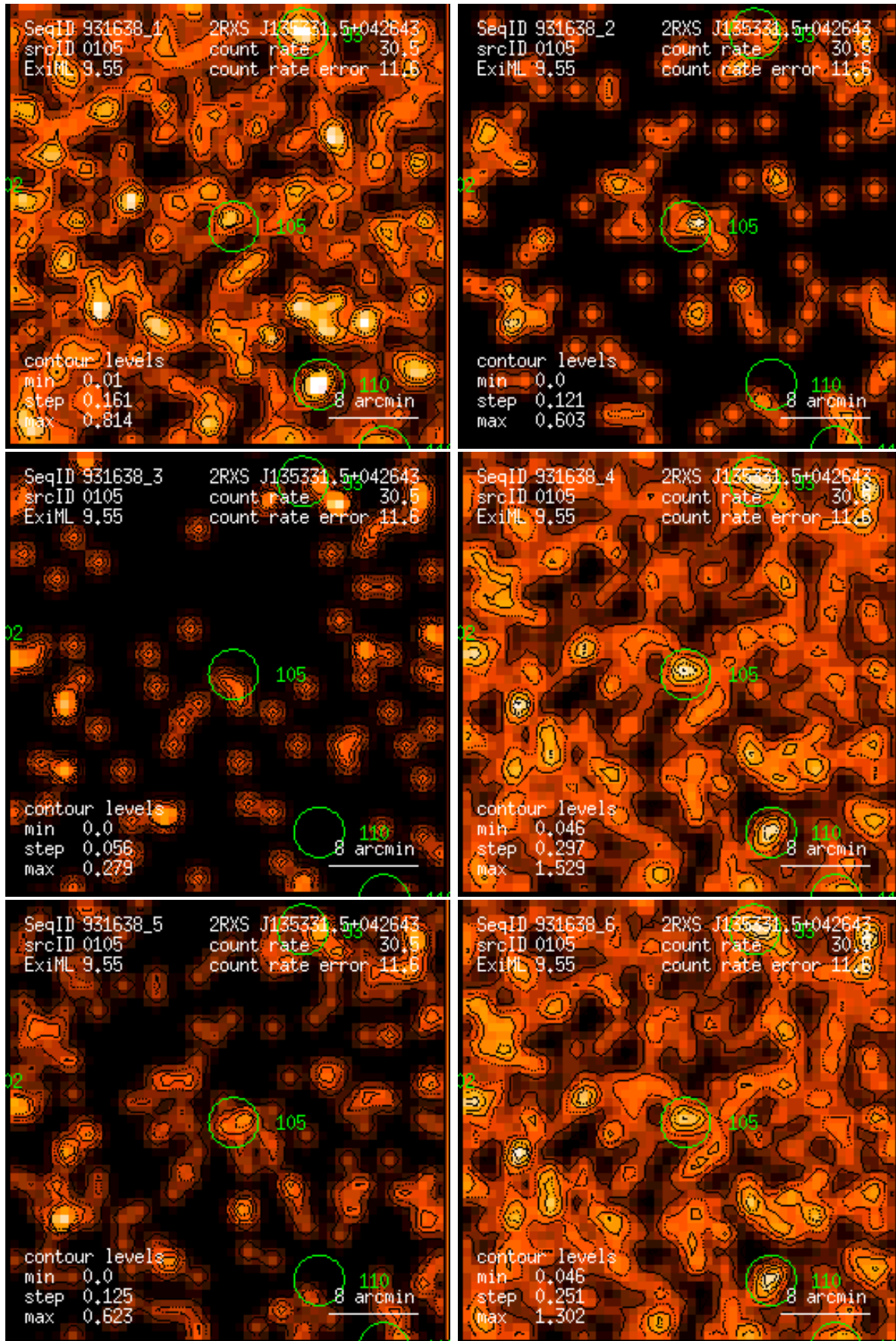
Figure 105: RASS 931638: detection 0105: band rate images, Gaussian filter: (1) PSPC channels 11 – 41, (2) 52 – 90, (3) 91 – 201, (4) 11 – 235, (5) 52 – 201, (6) 11 – 201. Broad band rates in counts/ks. Band rate contour levels in counts/ks/arcmin 2 .
