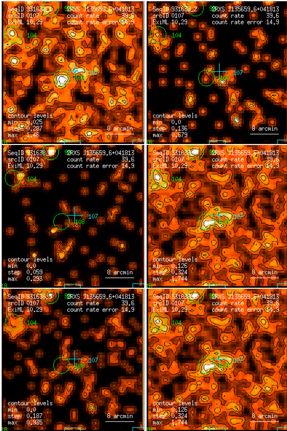
Figure 107: RASS 931638: detection 0107: band rate images, Gaussian filter: (1) PSPC channels 11 – 41, (2) 52 – 90, (3) 91 – 201, (4) 11 – 235, (5) 52 – 201, (6) 11 – 201. Broad band rates in counts/ks. Band rate contour levels in counts/ks/arcmin 2 .
