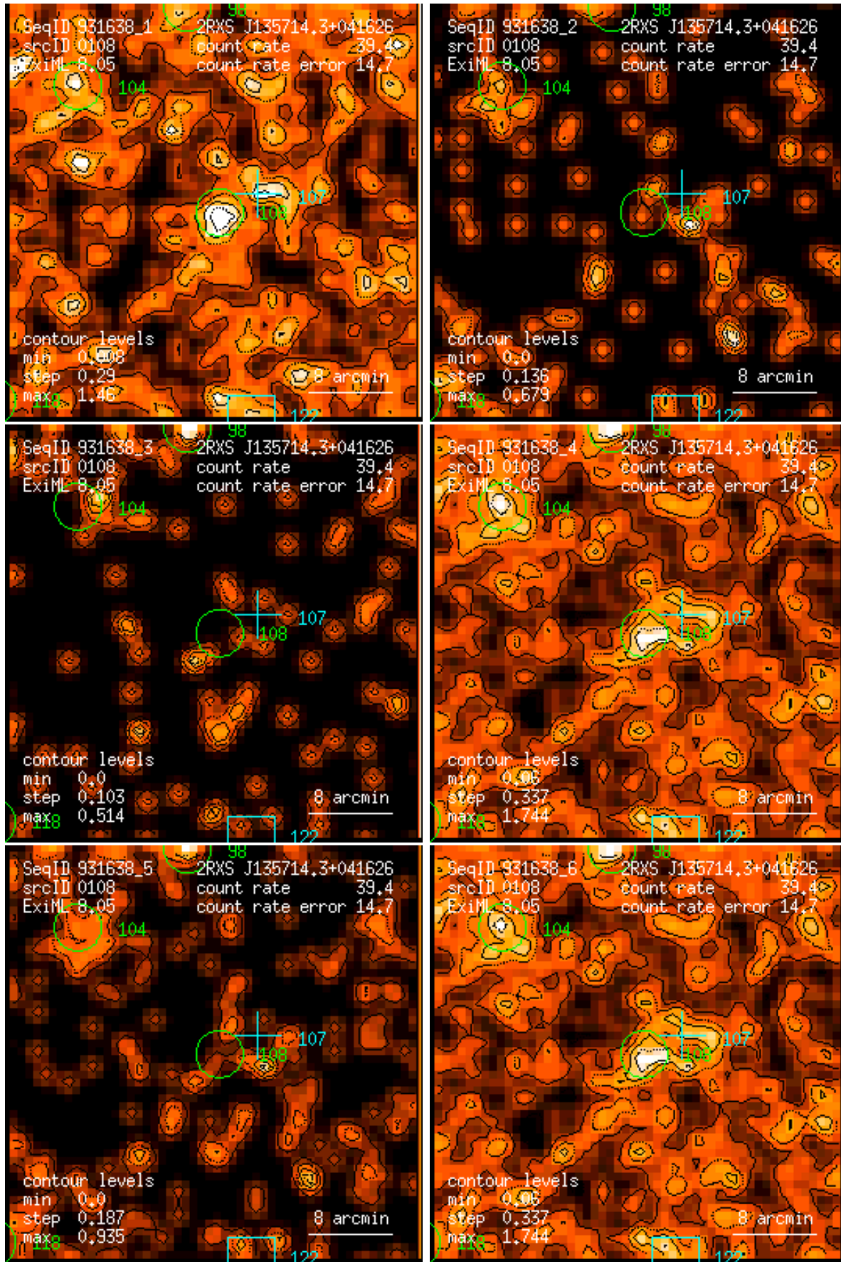
Figure 108: RASS 931638: detection 0108: band rate images, Gaussian filter: (1) PSPC channels 11 – 41, (2) 52 – 90, (3) 91 – 201, (4) 11 – 235, (5) 52 – 201, (6) 11 – 201. Broad band rates in counts/ks. Band rate contour levels in counts/ks/arcmin 2 .
