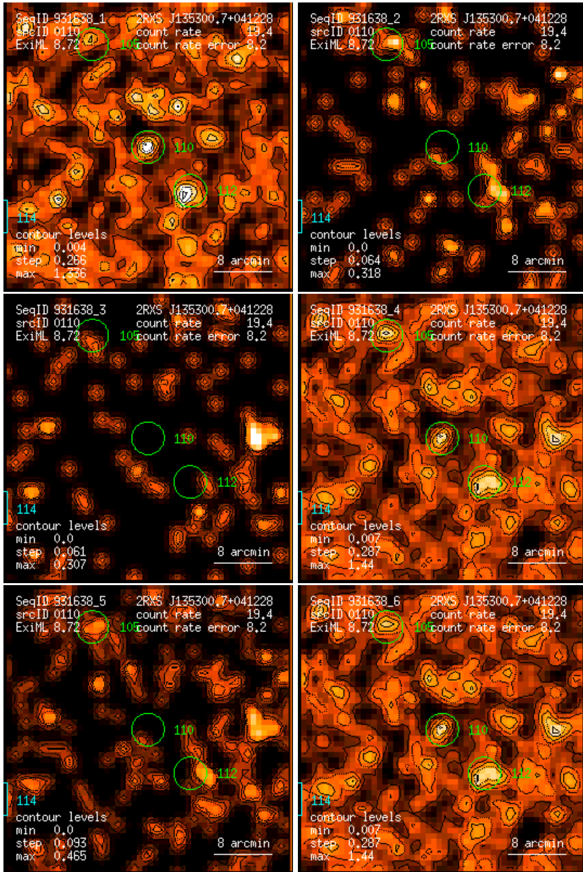
Figure 110: RASS 931638: detection 0110: band rate images, Gaussian filter: (1) PSPC channels 11 – 41, (2) 52 – 90, (3) 91 – 201, (4) 11 – 235, (5) 52 – 201, (6) 11 – 201. Broad band rates in counts/ks. Band rate contour levels in counts/ks/arcmin 2 .
