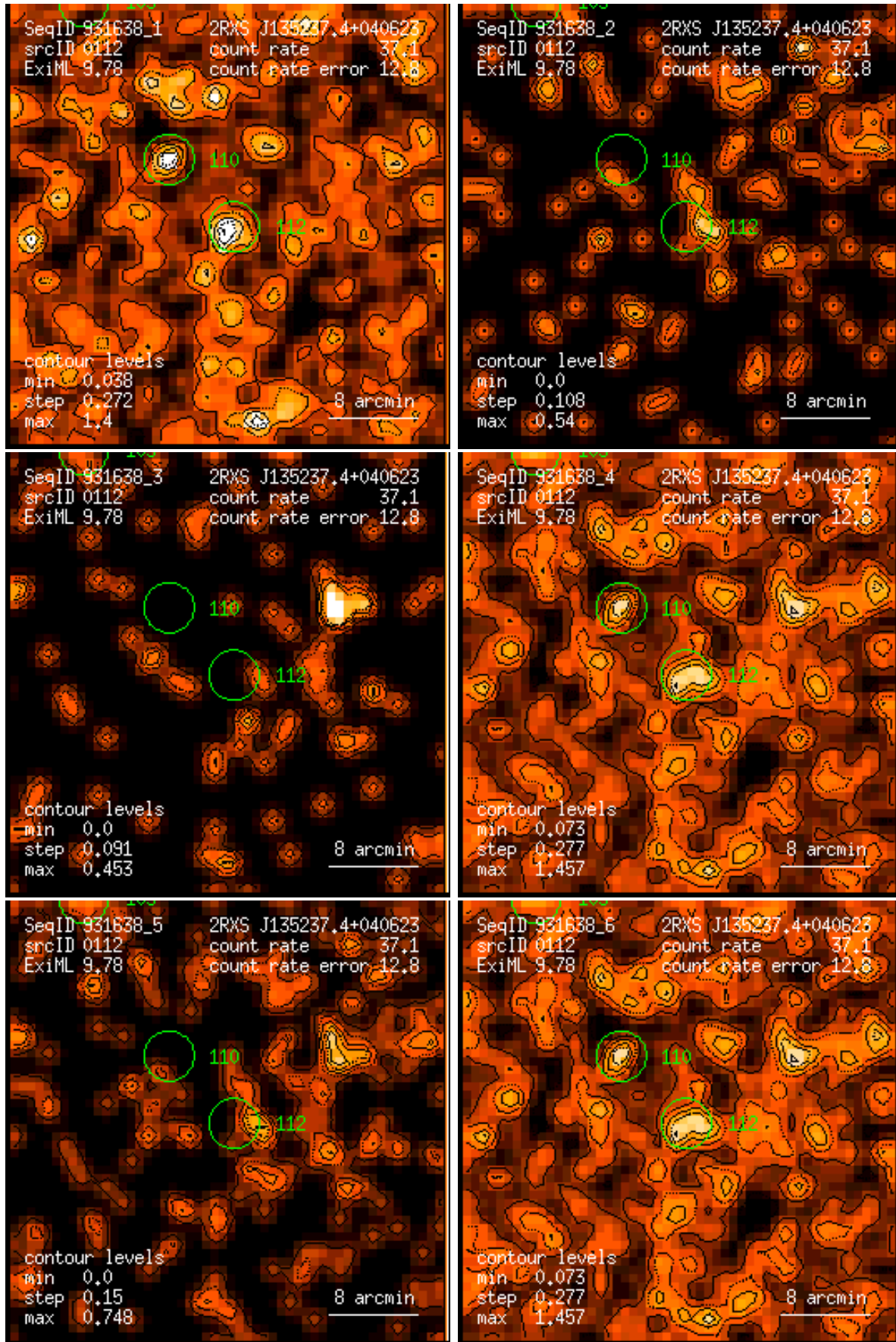
Figure 112: RASS 931638: detection 0112: band rate images, Gaussian filter: (1) PSPC channels 11 – 41, (2) 52 – 90, (3) 91 – 201, (4) 11 – 235, (5) 52 – 201, (6) 11 – 201. Broad band rates in counts/ks. Band rate contour levels in counts/ks/arcmin 2 .
