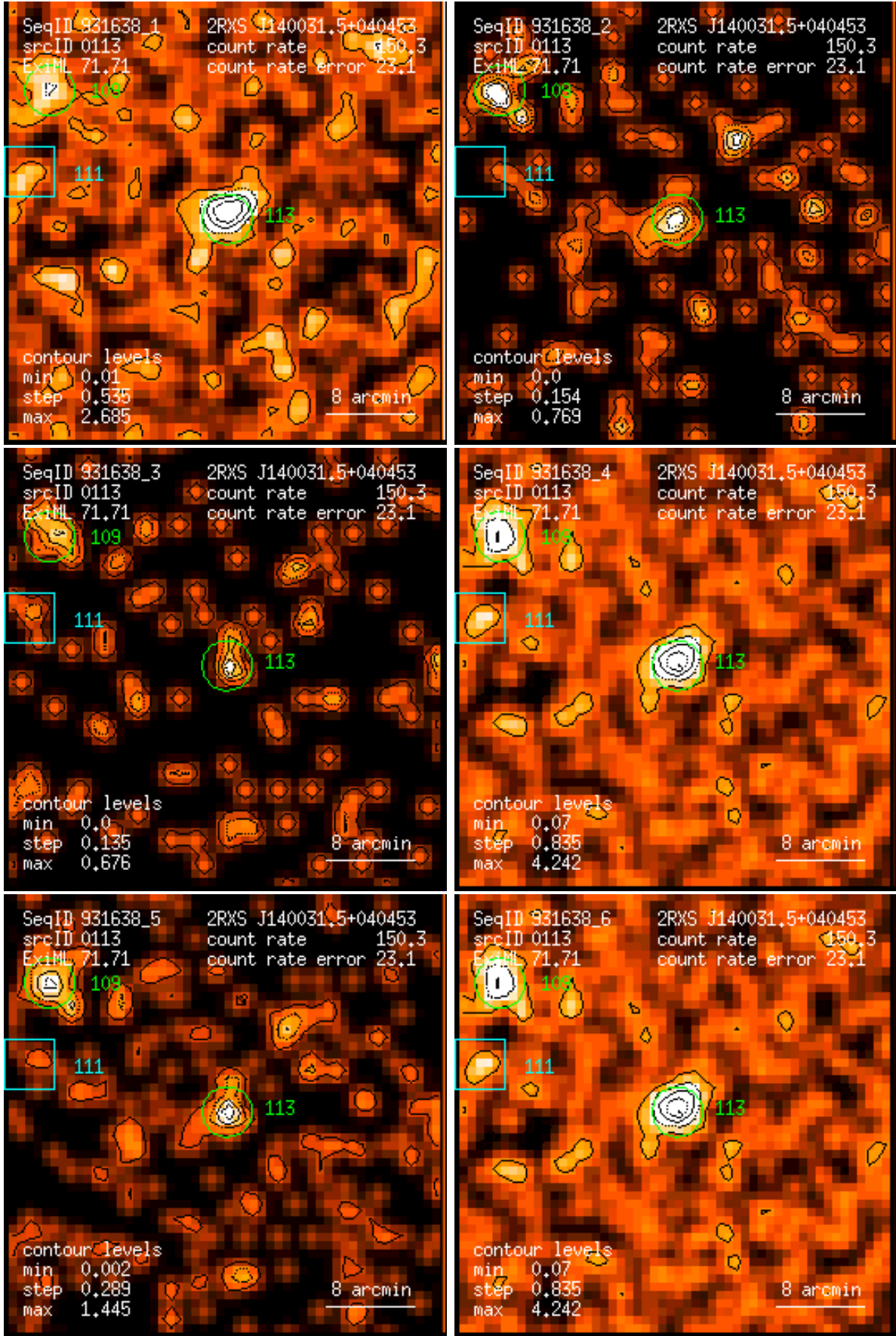
Figure 113: RASS 931638: detection 0113: band rate images, Gaussian filter: (1) PSPC channels 11 – 41, (2) 52 – 90, (3) 91 – 201, (4) 11 – 235, (5) 52 – 201, (6) 11 – 201. Broad band rates in counts/ks. Band rate contour levels in counts/ks/arcmin 2 .
