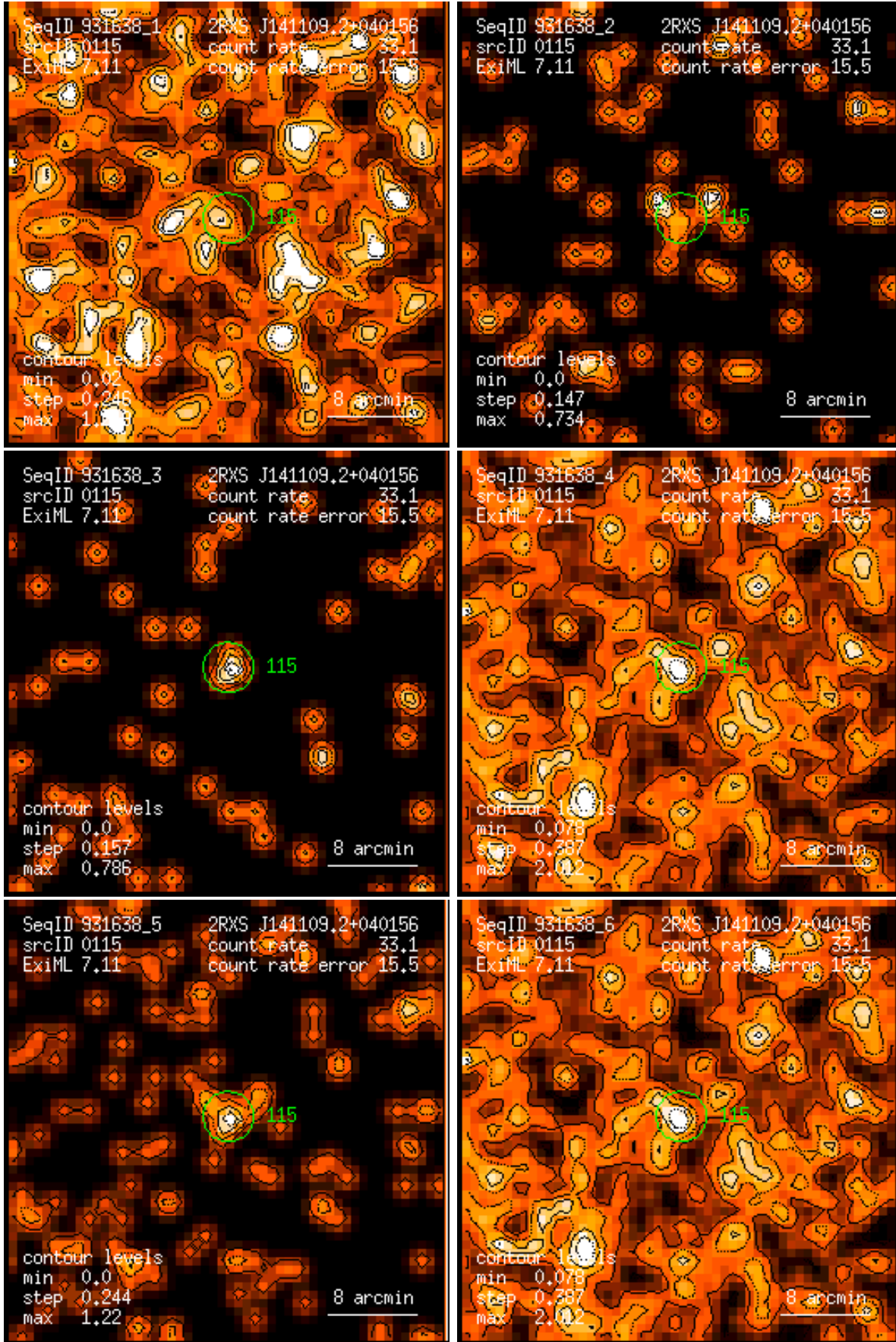
Figure 115: RASS 931638: detection 0115: band rate images, Gaussian filter: (1) PSPC channels 11 – 41, (2) 52 – 90, (3) 91 – 201, (4) 11 – 235, (5) 52 – 201, (6) 11 – 201. Broad band rates in counts/ks. Band rate contour levels in counts/ks/arcmin 2 .
