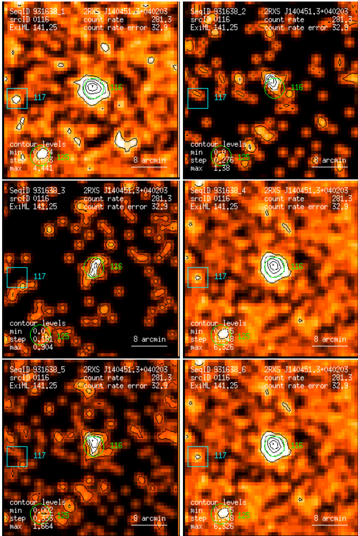
Figure 116: RASS 931638: detection 0116: band rate images, Gaussian filter: (1) PSPC channels 11 – 41, (2) 52 – 90, (3) 91 – 201, (4) 11 – 235, (5) 52 – 201, (6) 11 – 201. Broad band rates in counts/ks. Band rate contour levels in counts/ks/arcmin 2 .
