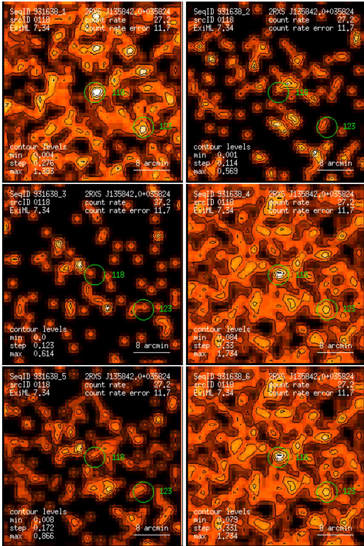
Figure 118: RASS 931638: detection 0118: band rate images, Gaussian filter: (1) PSPC channels 11 – 41, (2) 52 – 90, (3) 91 – 201, (4) 11 – 235, (5) 52 – 201, (6) 11 – 201. Broad band rates in counts/ks. Band rate contour levels in counts/ks/arcmin 2 .
