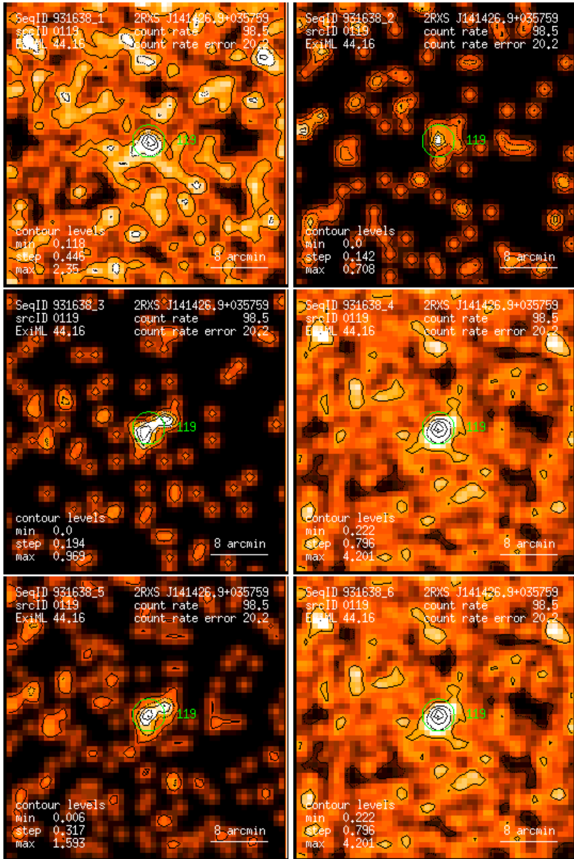
Figure 119: RASS 931638: detection 0119: band rate images, Gaussian filter: (1) PSPC channels 11 – 41, (2) 52 – 90, (3) 91 – 201, (4) 11 – 235, (5) 52 – 201, (6) 11 – 201. Broad band rates in counts/ks. Band rate contour levels in counts/ks/arcmin 2 .
