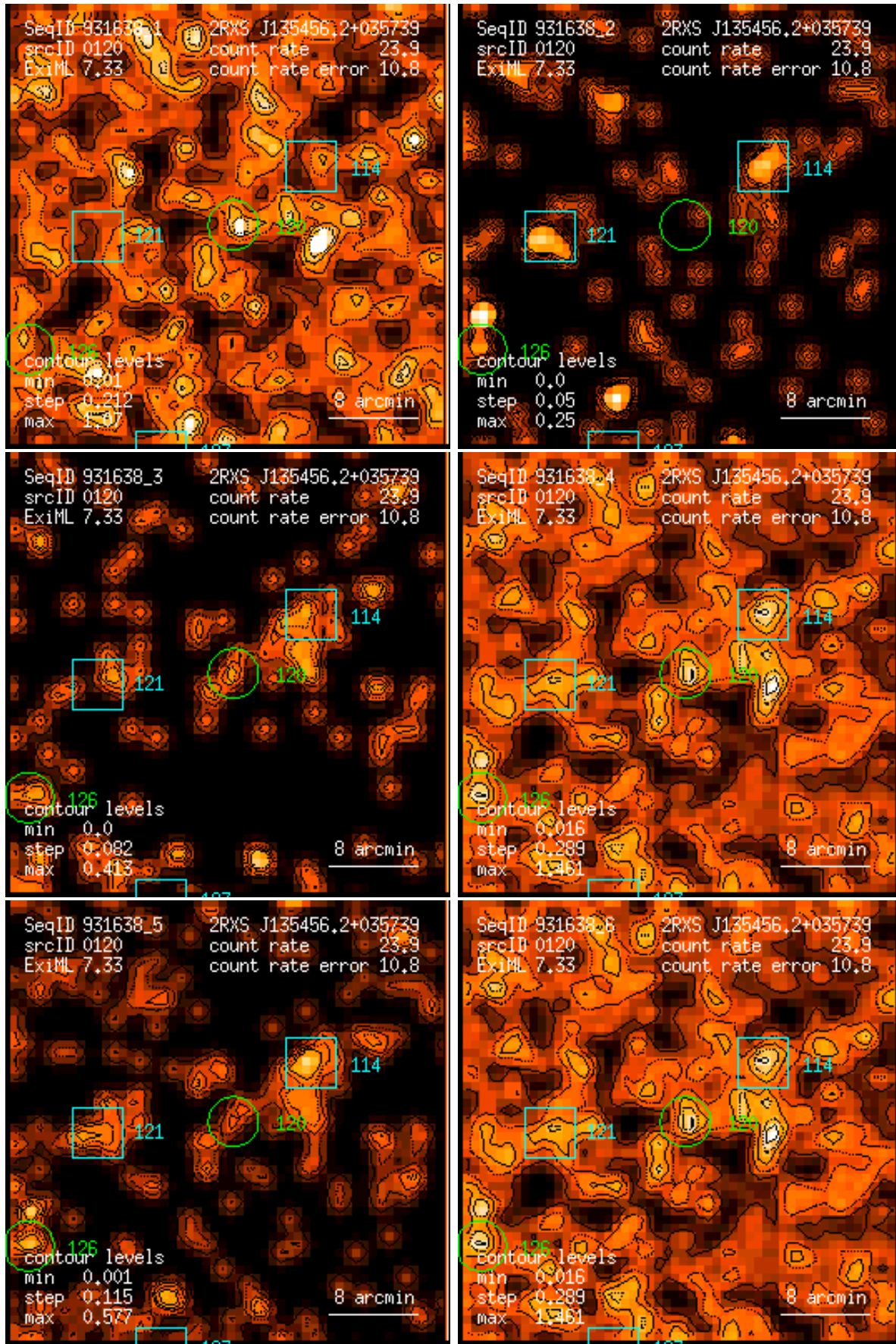
Figure 120: RASS 931638: detection 0120: band rate images, Gaussian filter: (1) PSPC channels 11 – 41, (2) 52 – 90, (3) 91 – 201, (4) 11 – 235, (5) 52 – 201, (6) 11 – 201. Broad band rates in counts/ks. Band rate contour levels in counts/ks/arcmin 2 .
