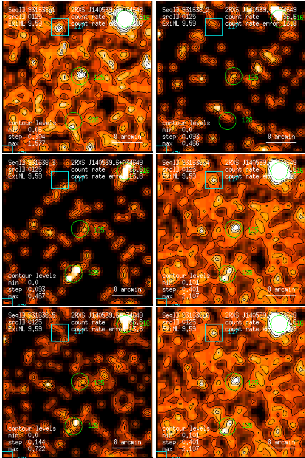
Figure 125: RASS 931638: detection 0125: band rate images, Gaussian filter: (1) PSPC channels 11 – 41, (2) 52 – 90, (3) 91 – 201, (4) 11 – 235, (5) 52 – 201, (6) 11 – 201. Broad band rates in counts/ks. Band rate contour levels in counts/ks/arcmin 2 .
