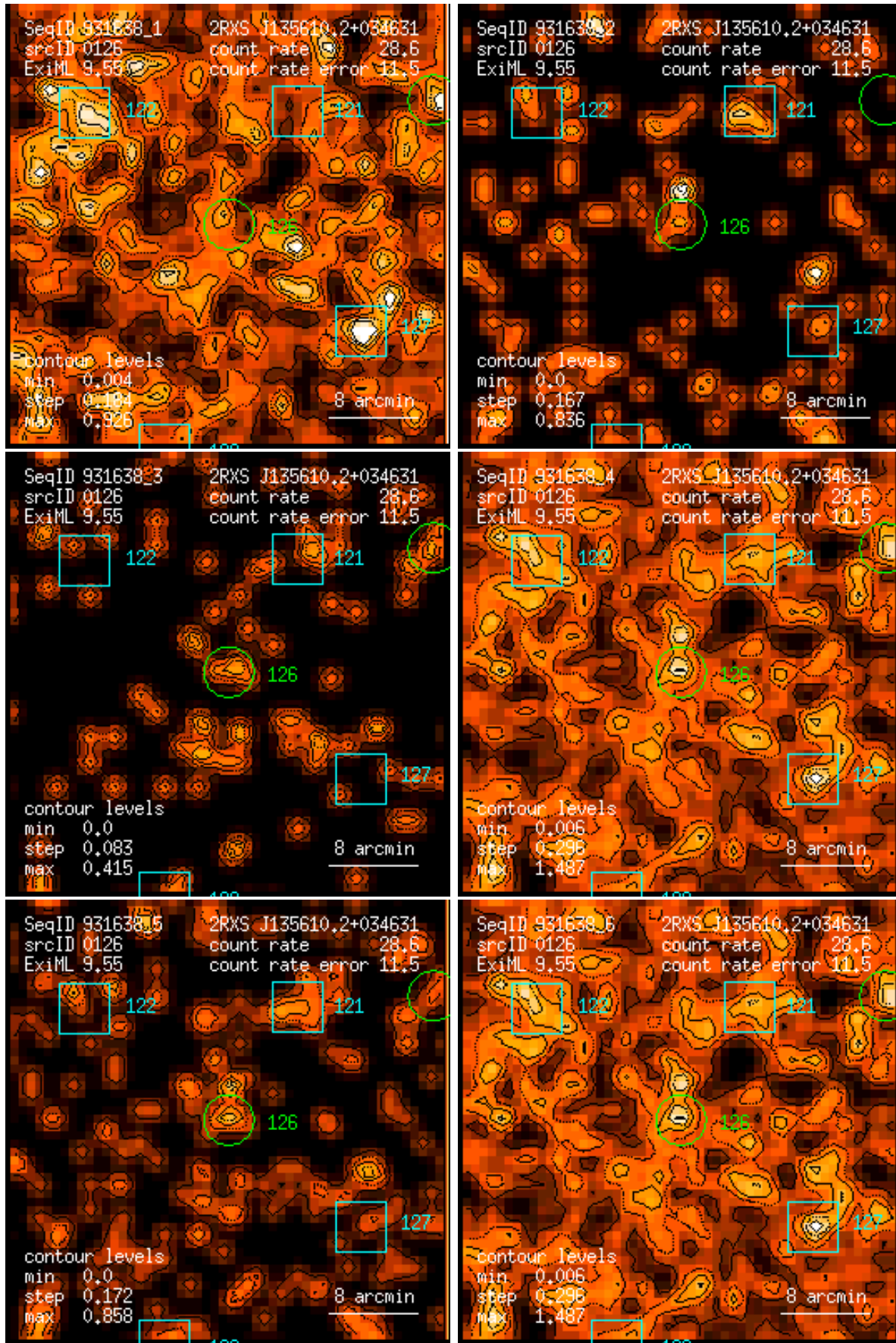
Figure 126: RASS 931638: detection 0126: band rate images, Gaussian filter: (1) PSPC channels 11 – 41, (2) 52 – 90, (3) 91 – 201, (4) 11 – 235, (5) 52 – 201, (6) 11 – 201. Broad band rates in counts/ks. Band rate contour levels in counts/ks/arcmin 2 .
