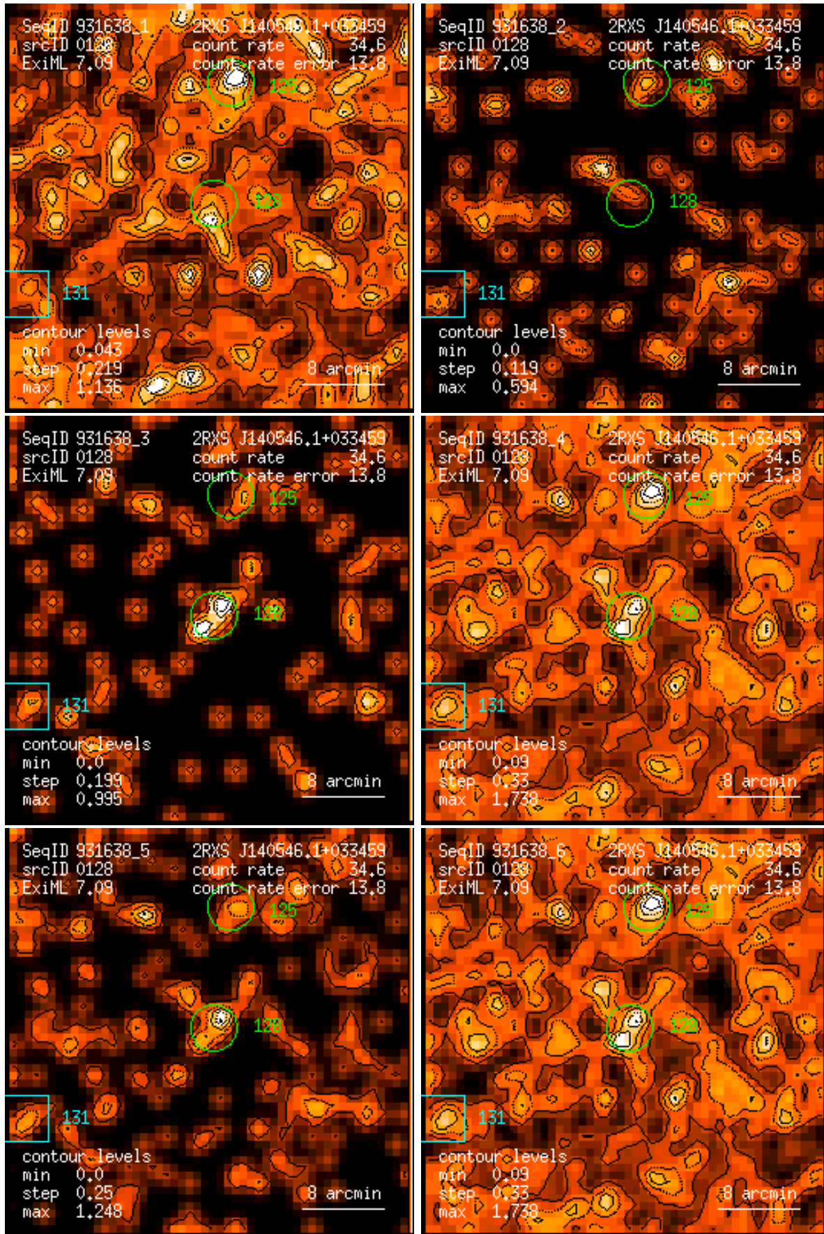
Figure 128: RASS 931638: detection 0128: band rate images, Gaussian filter: (1) PSPC channels 11 – 41, (2) 52 – 90, (3) 91 – 201, (4) 11 – 235, (5) 52 – 201, (6) 11 – 201. Broad band rates in counts/ks. Band rate contour levels in counts/ks/arcmin 2 .
