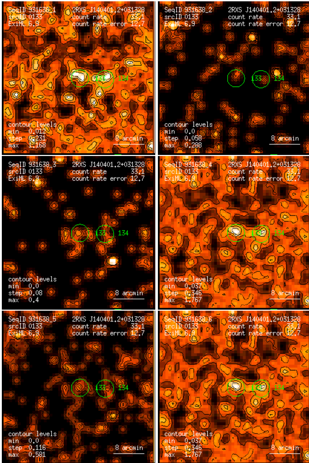
Figure 133: RASS 931638: detection 0133: band rate images, Gaussian filter: (1) PSPC channels 11 – 41, (2) 52 – 90, (3) 91 – 201, (4) 11 – 235, (5) 52 – 201, (6) 11 – 201. Broad band rates in counts/ks. Band rate contour levels in counts/ks/arcmin 2 .
