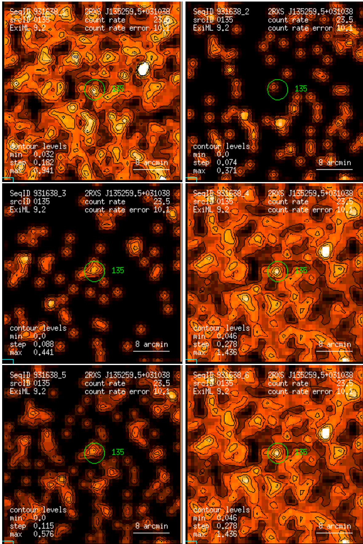
Figure 135: RASS 931638: detection 0135: band rate images, Gaussian filter: (1) PSPC channels 11 – 41, (2) 52 – 90, (3) 91 – 201, (4) 11 – 235, (5) 52 – 201, (6) 11 – 201. Broad band rates in counts/ks. Band rate contour levels in counts/ks/arcmin 2 .
