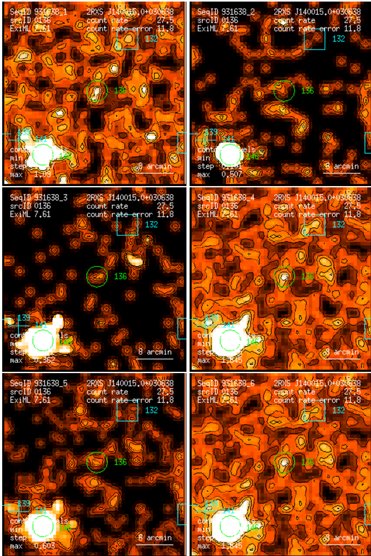
Figure 136: RASS 931638: detection 0136: band rate images, Gaussian filter: (1) PSPC channels 11 – 41, (2) 52 – 90, (3) 91 – 201, (4) 11 – 235, (5) 52 – 201, (6) 11 – 201. Broad band rates in counts/ks. Band rate contour levels in counts/ks/arcmin 2 .
