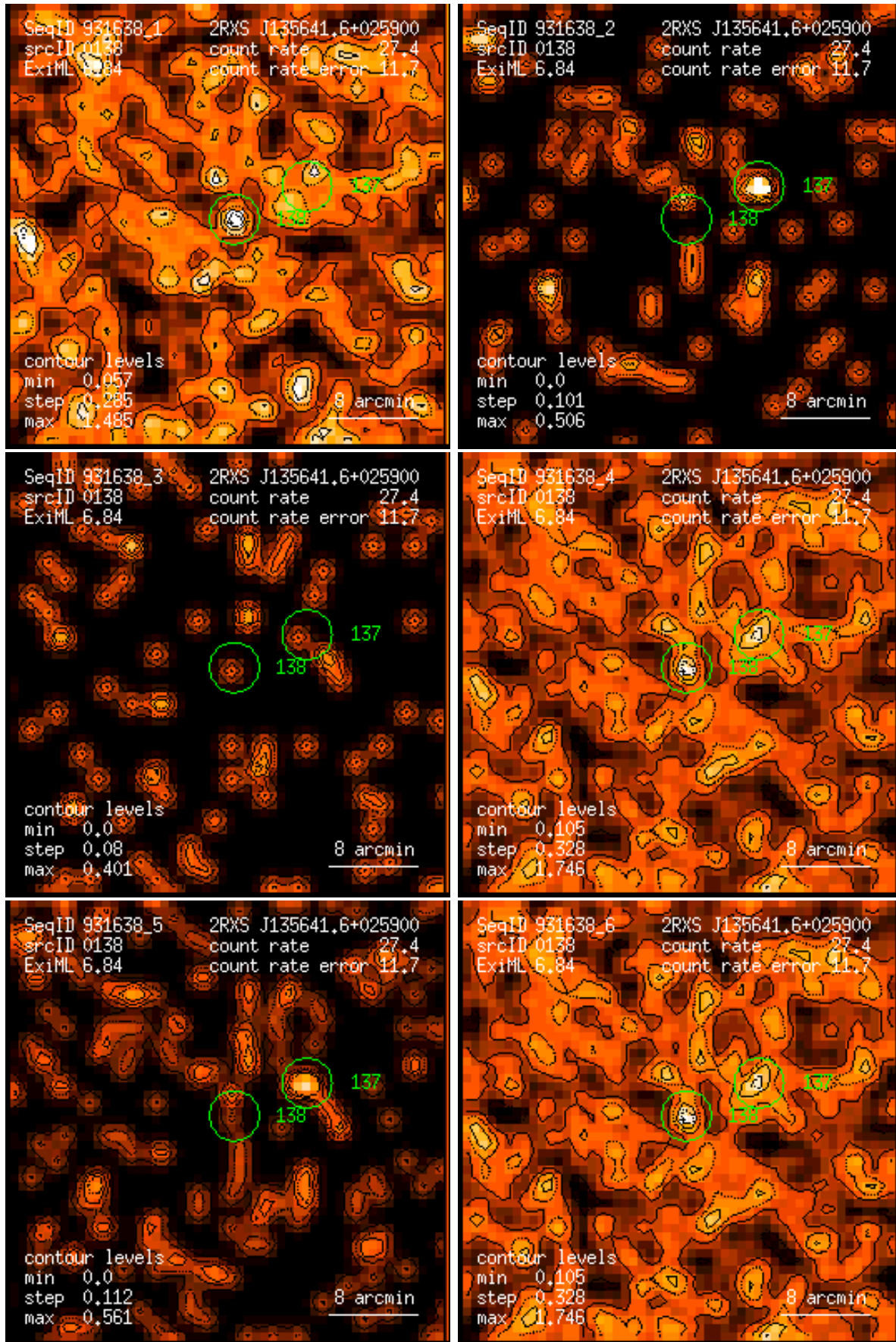
Figure 138: RASS 931638: detection 0138: band rate images, Gaussian filter: (1) PSPC channels 11 – 41, (2) 52 – 90, (3) 91 – 201, (4) 11 – 235, (5) 52 – 201, (6) 11 – 201. Broad band rates in counts/ks. Band rate contour levels in counts/ks/arcmin 2 .
