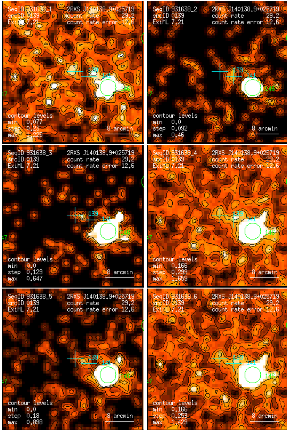
Figure 139: RASS 931638: detection 0139: band rate images, Gaussian filter: (1) PSPC channels 11 – 41, (2) 52 – 90, (3) 91 – 201, (4) 11 – 235, (5) 52 – 201, (6) 11 – 201. Broad band rates in counts/ks. Band rate contour levels in counts/ks/arcmin 2 .
