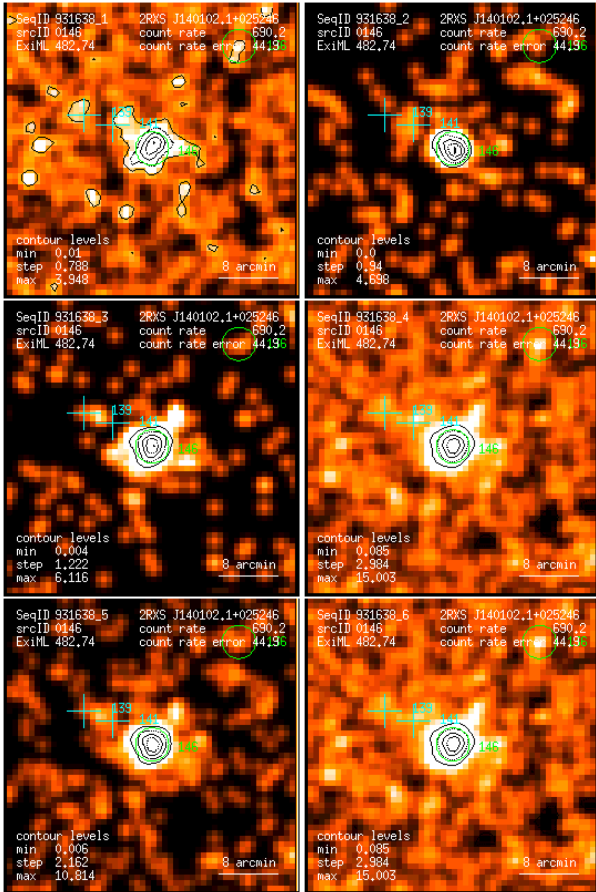
Figure 146: RASS 931638: detection 0146: band rate images, Gaussian filter: (1) PSPC channels 11 – 41, (2) 52 – 90, (3) 91 – 201, (4) 11 – 235, (5) 52 – 201, (6) 11 – 201. Broad band rates in counts/ks. Band rate contour levels in counts/ks/arcmin 2 .
