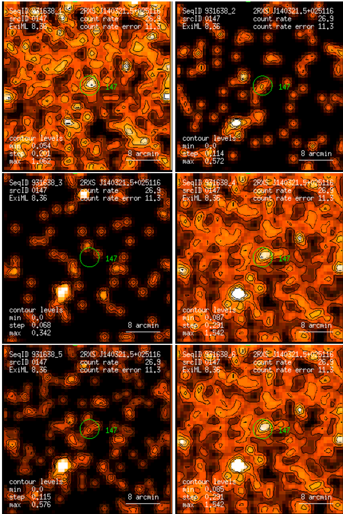
Figure 147: RASS 931638: detection 0147: band rate images, Gaussian filter: (1) PSPC channels 11 – 41, (2) 52 – 90, (3) 91 – 201, (4) 11 – 235, (5) 52 – 201, (6) 11 – 201. Broad band rates in counts/ks. Band rate contour levels in counts/ks/arcmin 2 .
