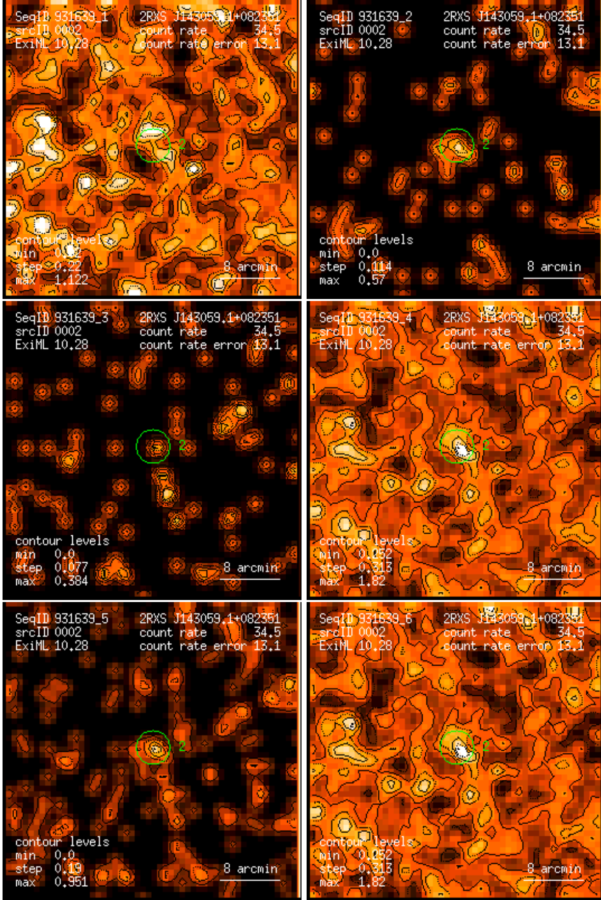
Figure 2: RASS 931639: detection 0002: band rate images, Gaussian filter: (1) PSPC channels 11 – 41, (2) 52 – 90, (3) 91 – 201, (4) 11 – 235, (5) 52 – 201, (6) 11 – 201. Broad band rates in counts/ks. Band rate contour levels in counts/ks/arcmin 2 .
