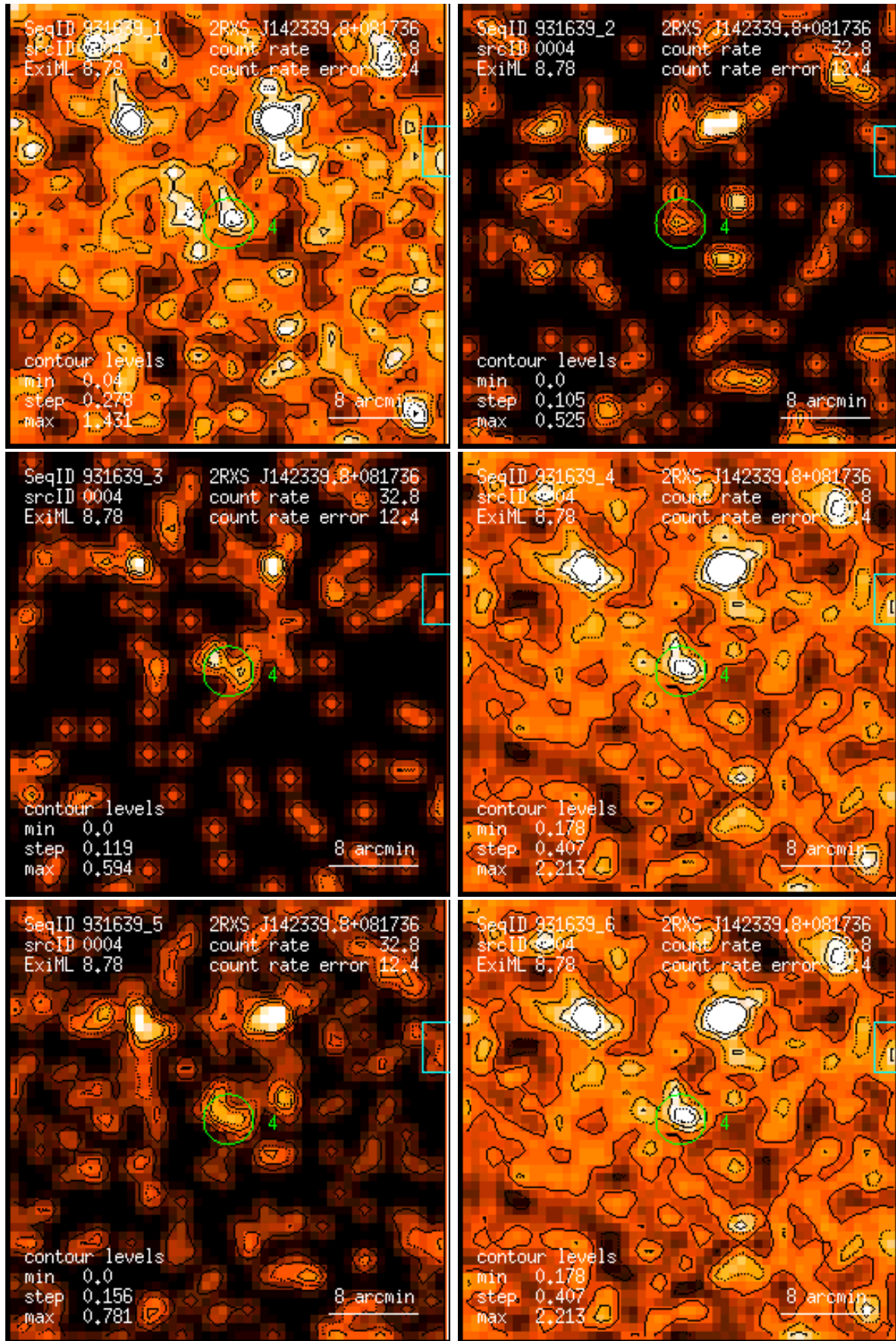
Figure 4: RASS 931639: detection 0004: band rate images, Gaussian filter: (1) PSPC channels 11 – 41, (2) 52 – 90, (3) 91 – 201, (4) 11 – 235, (5) 52 – 201, (6) 11 – 201. Broad band rates in counts/ks. Band rate contour levels in counts/ks/arcmin 2 .
