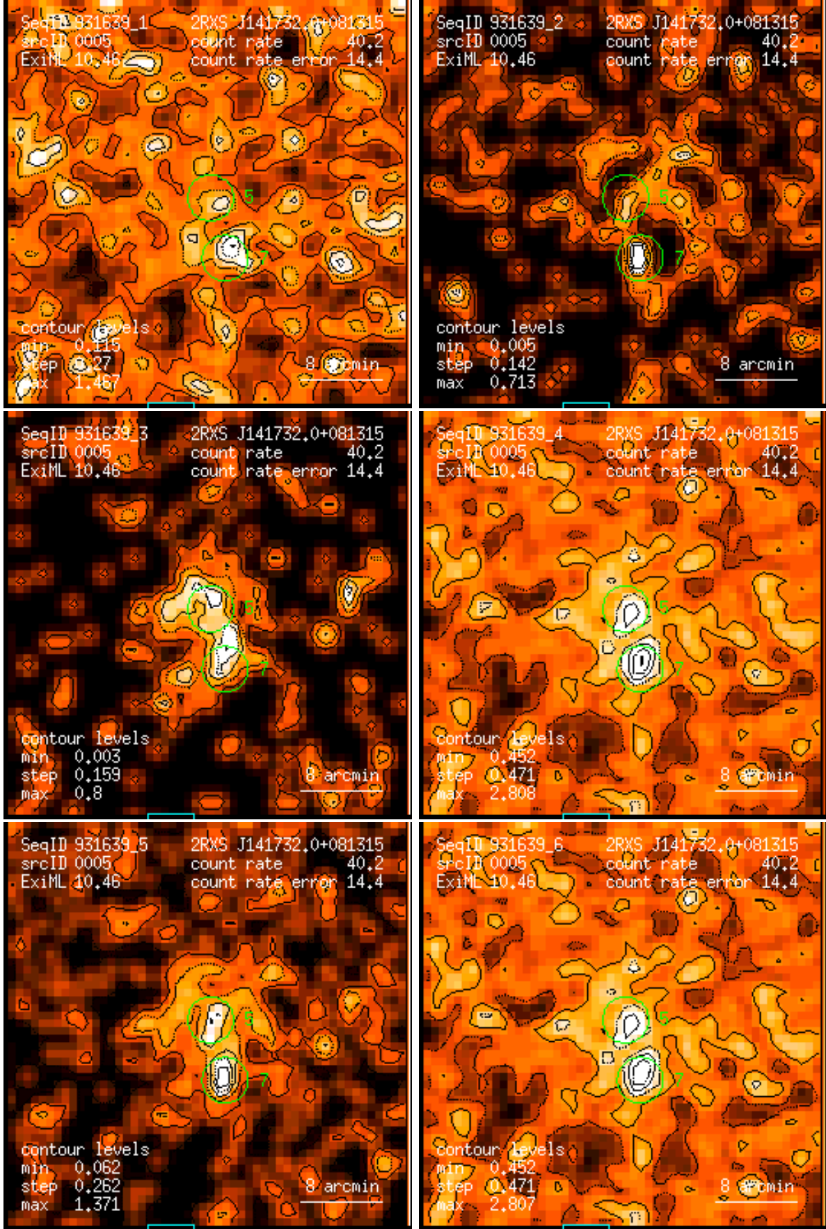
Figure 5: RASS 931639: detection 0005: band rate images, Gaussian filter: (1) PSPC channels 11 – 41, (2) 52 – 90, (3) 91 – 201, (4) 11 – 235, (5) 52 – 201, (6) 11 – 201. Broad band rates in counts/ks. Band rate contour levels in counts/ks/arcmin 2 .
