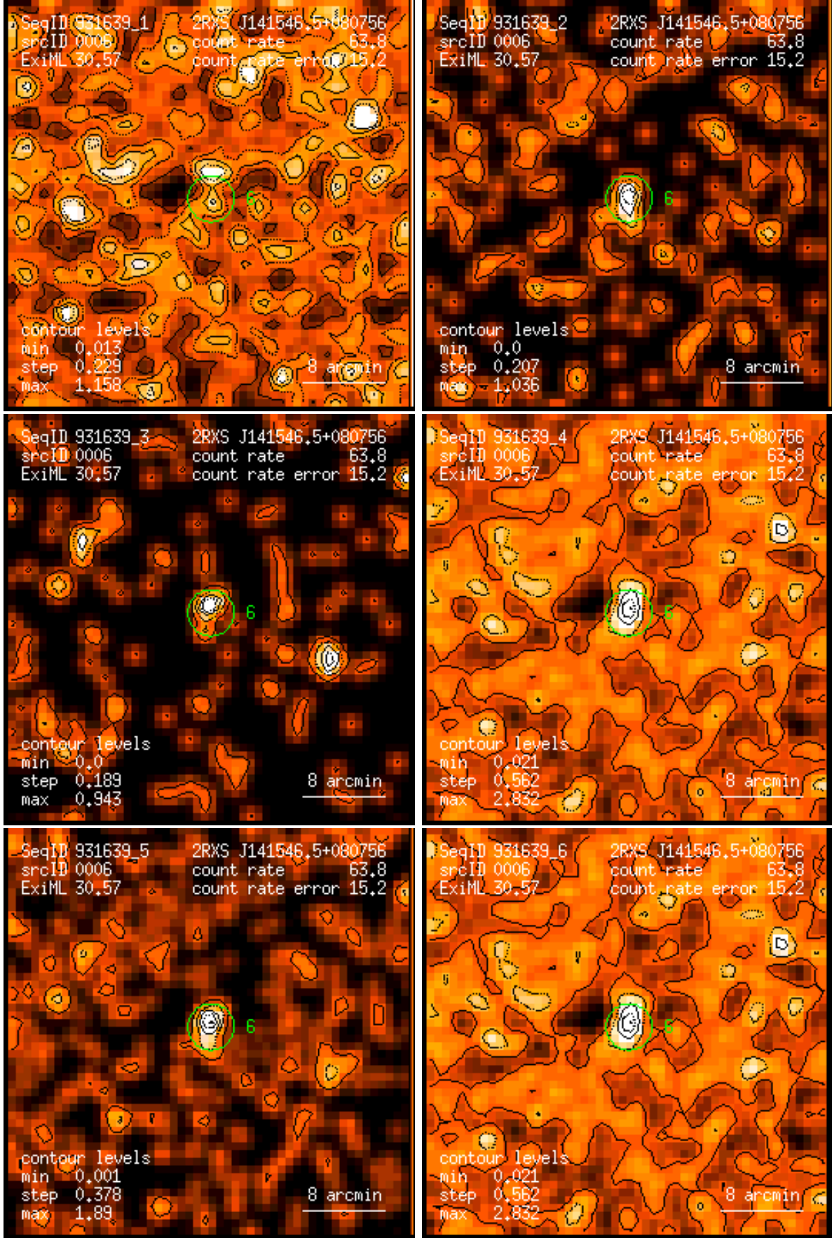
Figure 6: RASS 931639: detection 0006: band rate images, Gaussian filter: (1) PSPC channels 11 – 41, (2) 52 – 90, (3) 91 – 201, (4) 11 – 235, (5) 52 – 201, (6) 11 – 201. Broad band rates in counts/ks. Band rate contour levels in counts/ks/arcmin 2 .
