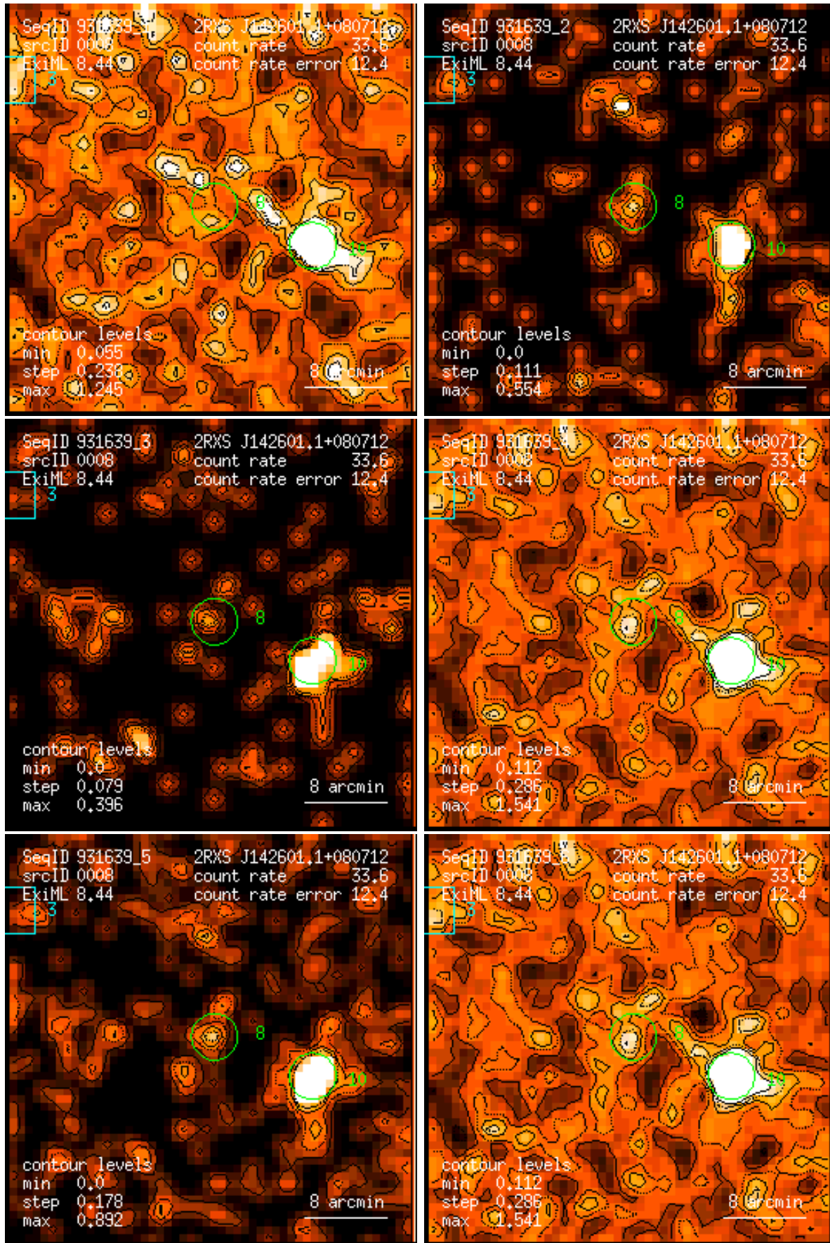
Figure 8: RASS 931639: detection 0008: band rate images, Gaussian filter: (1) PSPC channels 11 – 41, (2) 52 – 90, (3) 91 – 201, (4) 11 – 235, (5) 52 – 201, (6) 11 – 201. Broad band rates in counts/ks. Band rate contour levels in counts/ks/arcmin 2 .
