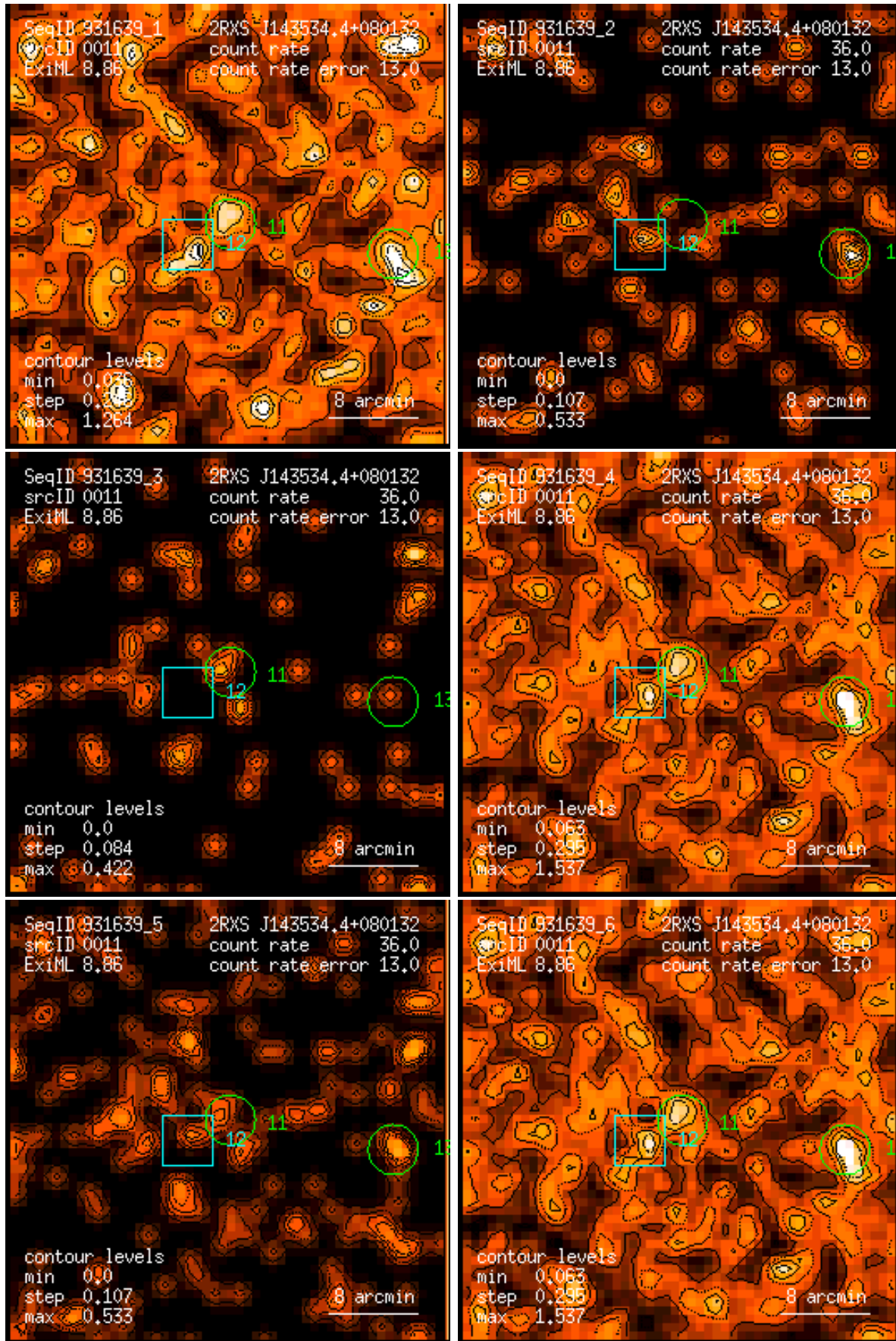
Figure 11: RASS 931639: detection 0011: band rate images, Gaussian filter: (1) PSPC channels 11 – 41, (2) 52 – 90, (3) 91 – 201, (4) 11 – 235, (5) 52 – 201, (6) 11 – 201. Broad band rates in counts/ks. Band rate contour levels in counts/ks/arcmin 2 .
