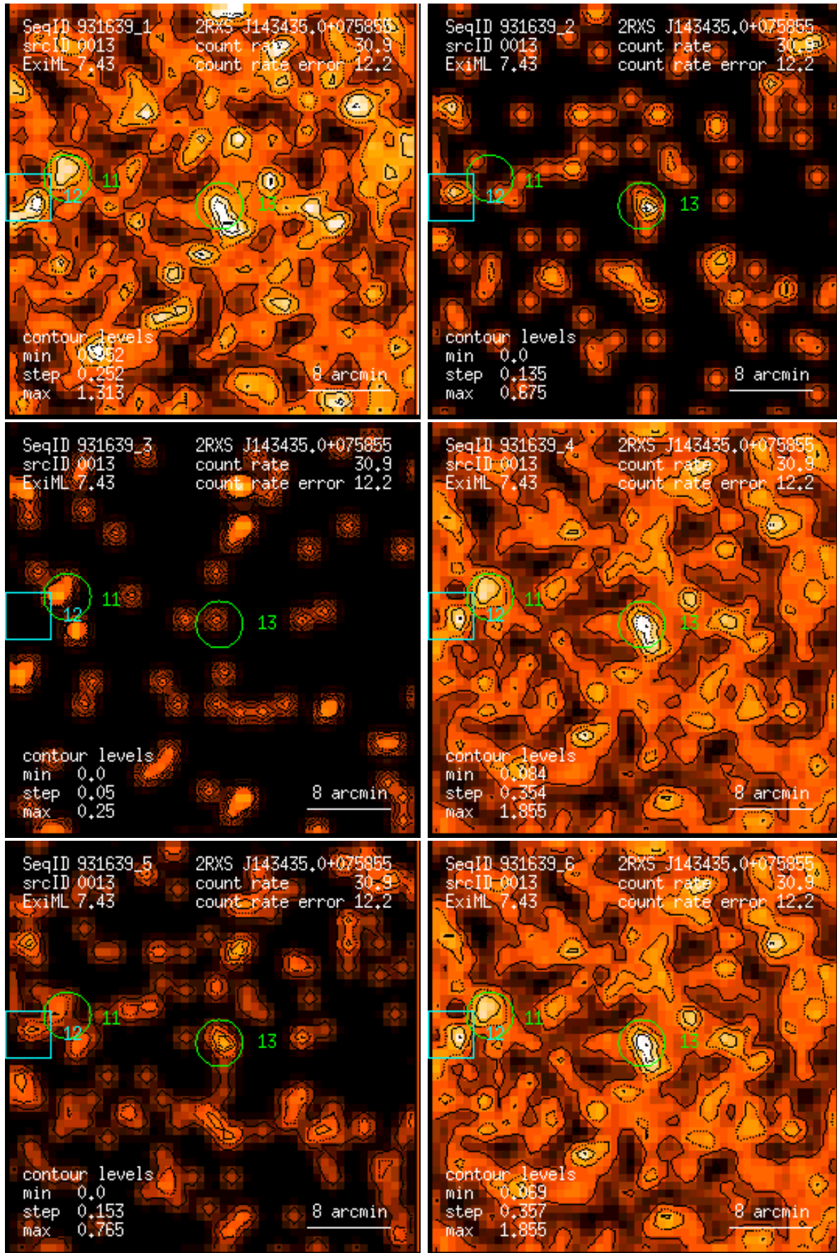
Figure 13: RASS 931639: detection 0013: band rate images, Gaussian filter: (1) PSPC channels 11 – 41, (2) 52 – 90, (3) 91 – 201, (4) 11 – 235, (5) 52 – 201, (6) 11 – 201. Broad band rates in counts/ks. Band rate contour levels in counts/ks/arcmin 2 .
