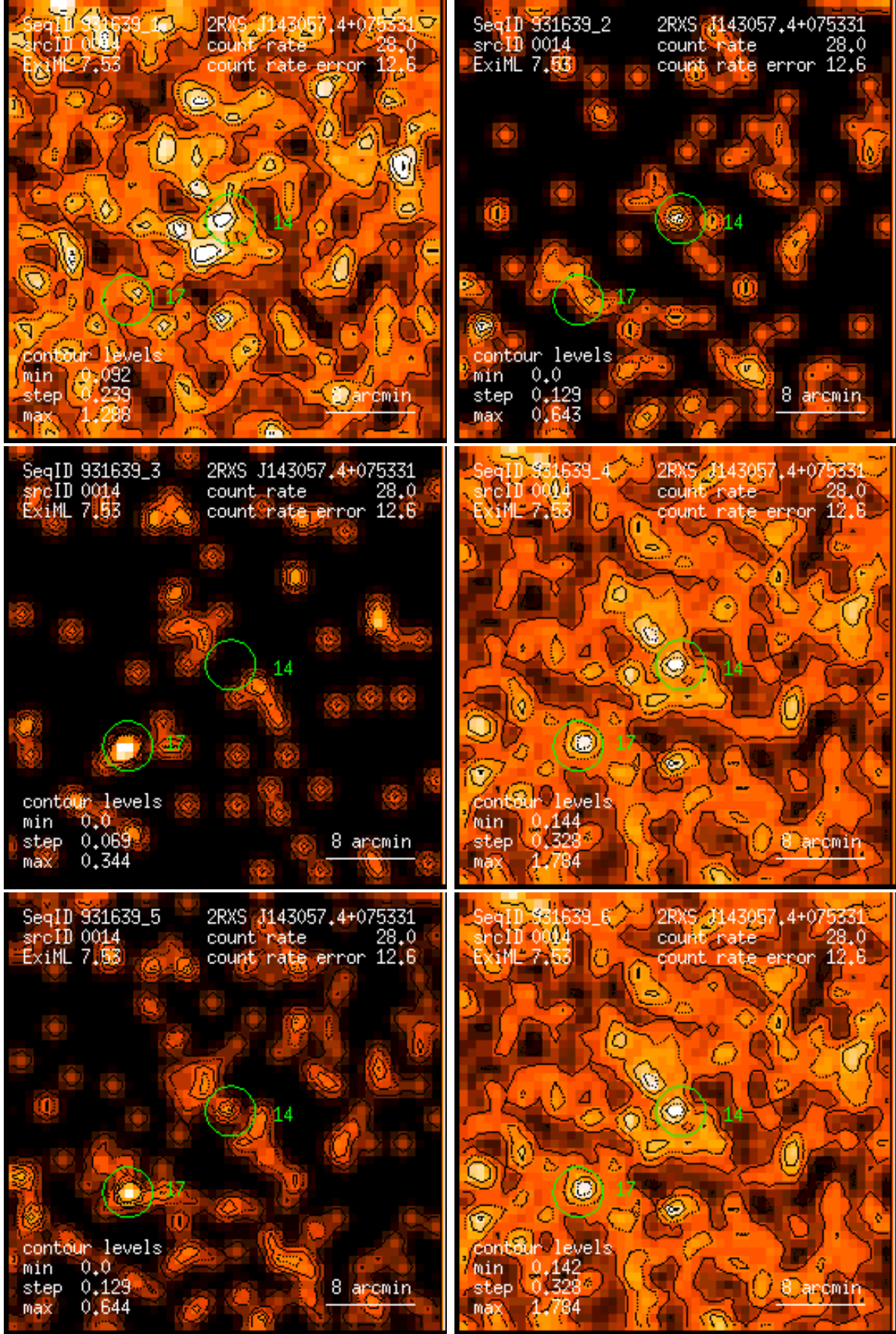
Figure 14: RASS 931639: detection 0014: band rate images, Gaussian filter: (1) PSPC channels 11 – 41, (2) 52 – 90, (3) 91 – 201, (4) 11 – 235, (5) 52 – 201, (6) 11 – 201. Broad band rates in counts/ks. Band rate contour levels in counts/ks/arcmin 2 .
