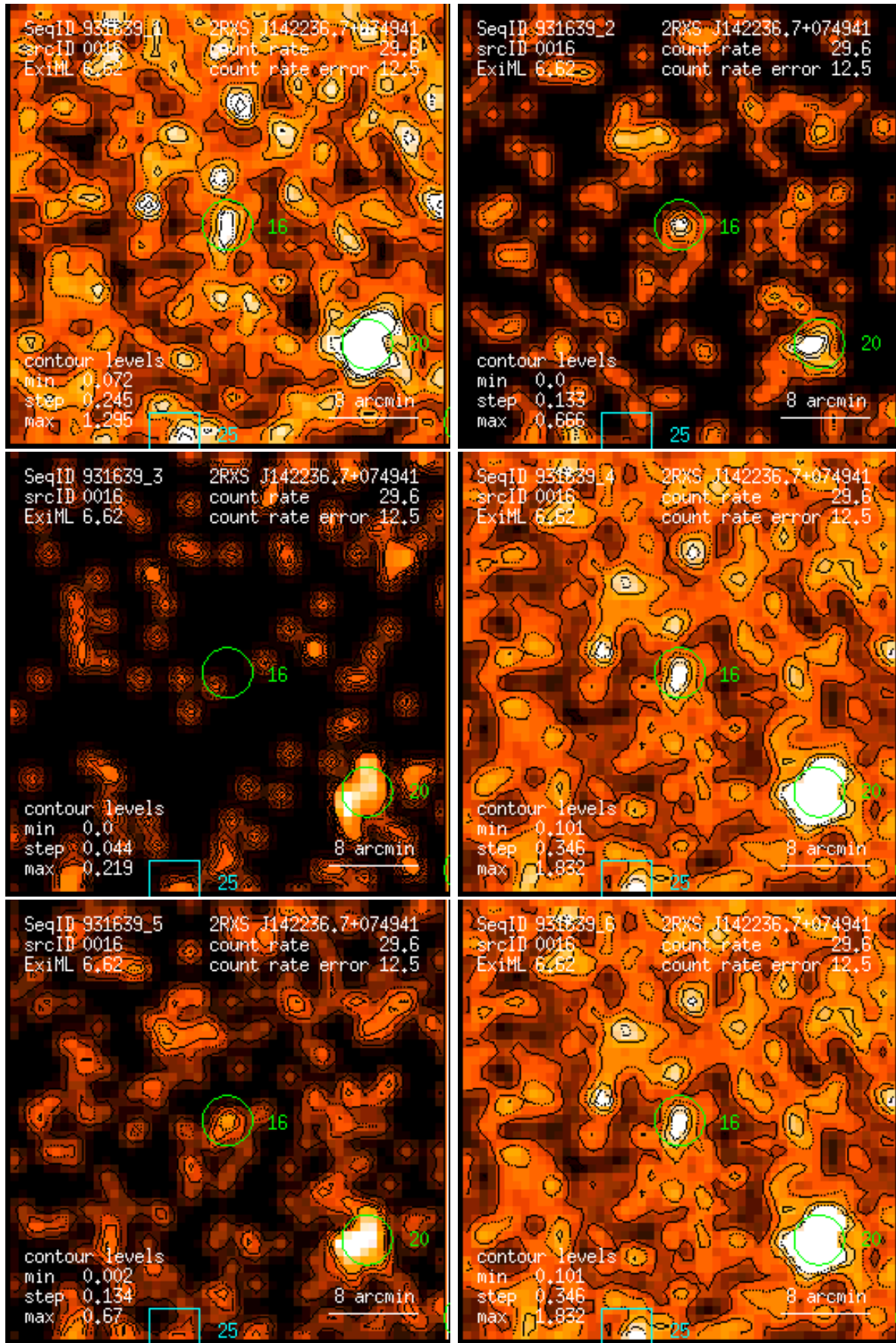
Figure 16: RASS 931639: detection 0016: band rate images, Gaussian filter: (1) PSPC channels 11 – 41, (2) 52 – 90, (3) 91 – 201, (4) 11 – 235, (5) 52 – 201, (6) 11 – 201. Broad band rates in counts/ks. Band rate contour levels in counts/ks/arcmin 2 .
