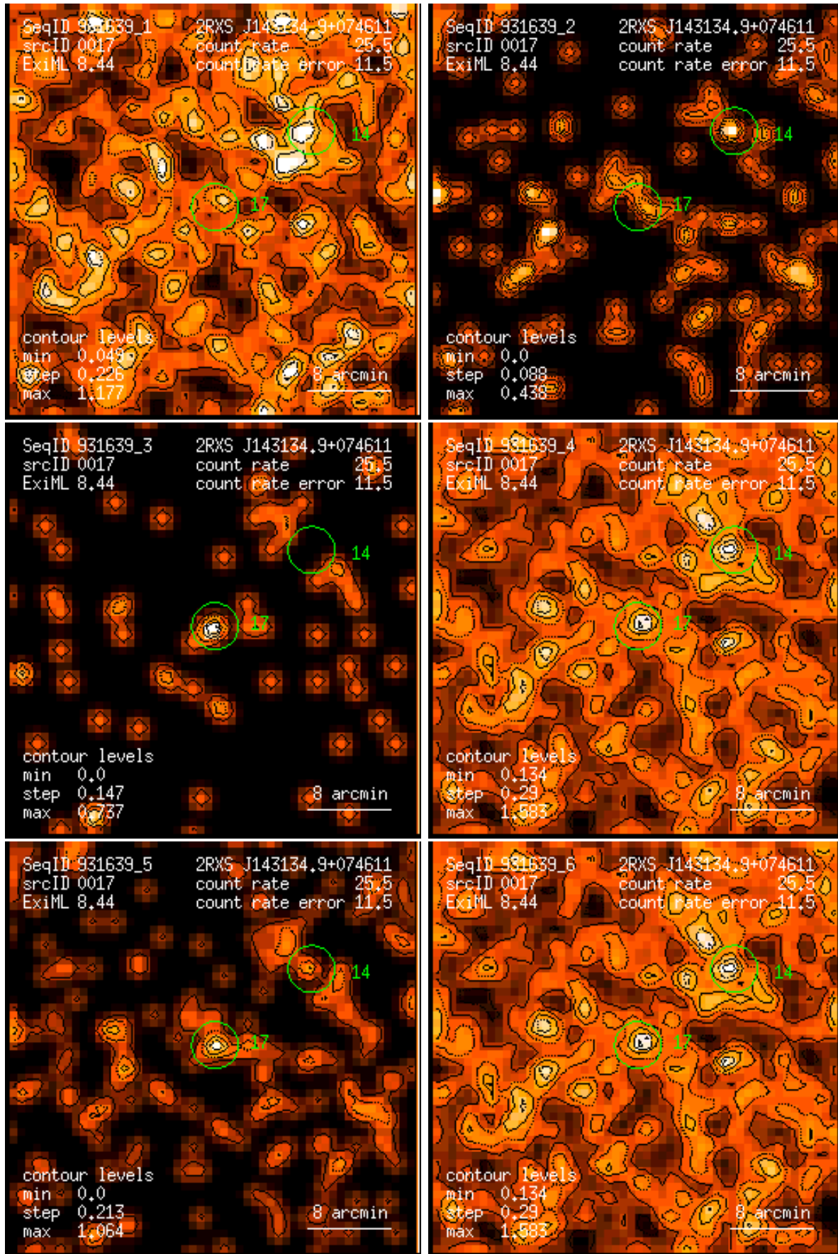
Figure 17: RASS 931639: detection 0017: band rate images, Gaussian filter: (1) PSPC channels 11 – 41, (2) 52 – 90, (3) 91 – 201, (4) 11 – 235, (5) 52 – 201, (6) 11 – 201. Broad band rates in counts/ks. Band rate contour levels in counts/ks/arcmin 2 .
