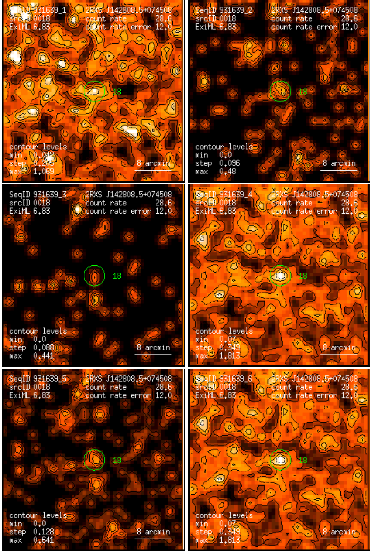
Figure 18: RASS 931639: detection 0018: band rate images, Gaussian filter: (1) PSPC channels 11 – 41, (2) 52 – 90, (3) 91 – 201, (4) 11 – 235, (5) 52 – 201, (6) 11 – 201. Broad band rates in counts/ks. Band rate contour levels in counts/ks/arcmin 2 .
