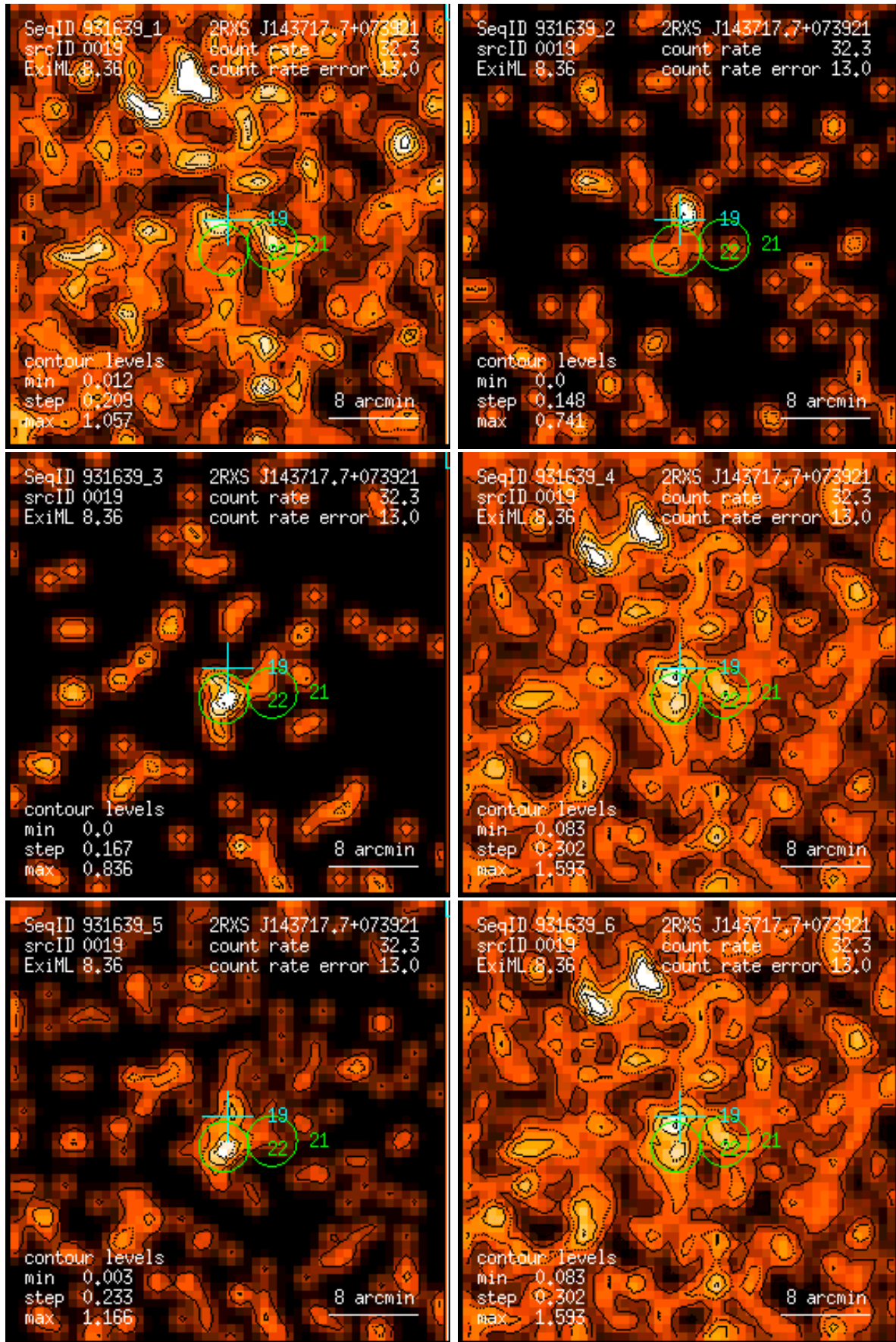
Figure 19: RASS 931639: detection 0019: band rate images, Gaussian filter: (1) PSPC channels 11 – 41, (2) 52 – 90, (3) 91 – 201, (4) 11 – 235, (5) 52 – 201, (6) 11 – 201. Broad band rates in counts/ks. Band rate contour levels in counts/ks/arcmin 2 .
