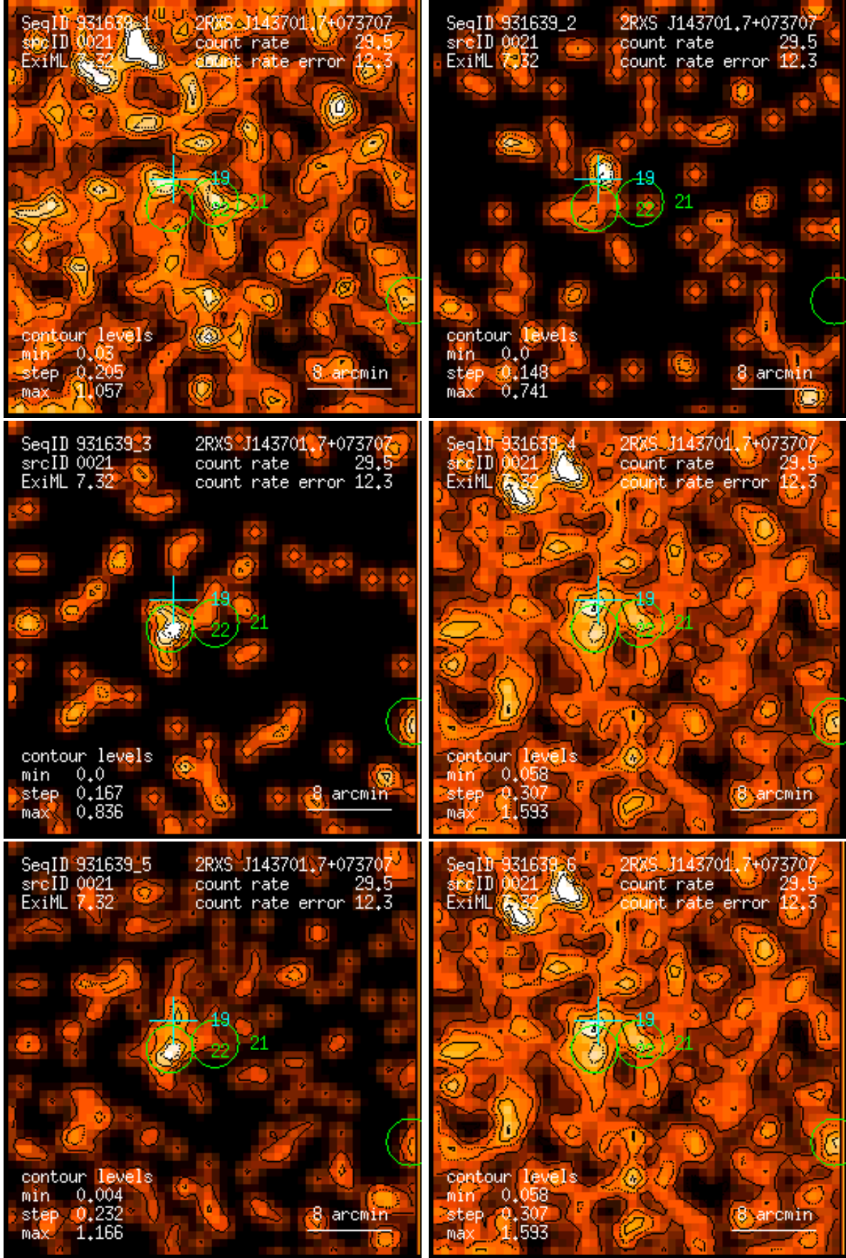
Figure 21: RASS 931639: detection 0021: band rate images, Gaussian filter: (1) PSPC channels 11 – 41, (2) 52 – 90, (3) 91 – 201, (4) 11 – 235, (5) 52 – 201, (6) 11 – 201. Broad band rates in counts/ks. Band rate contour levels in counts/ks/arcmin 2 .
