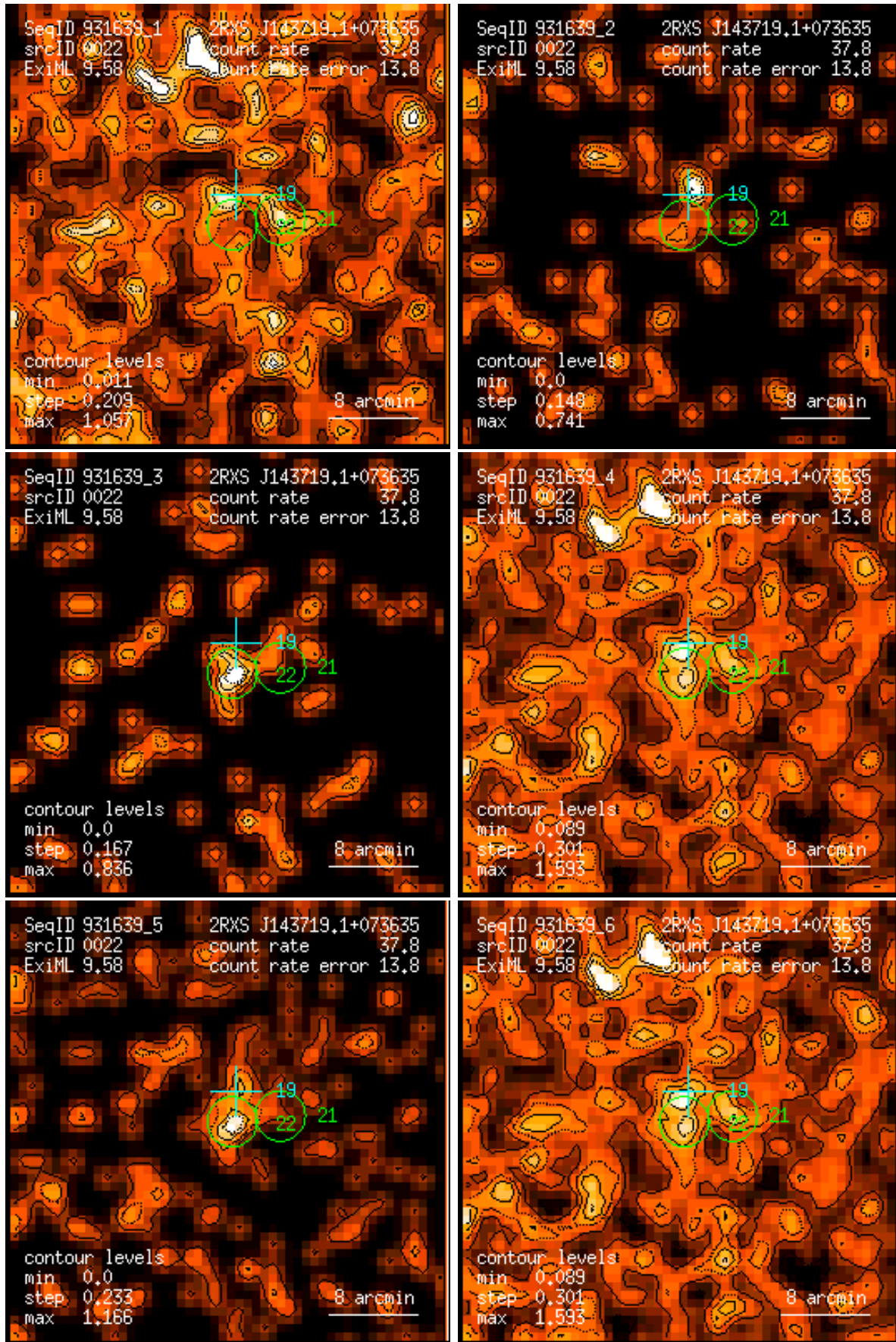
Figure 22: RASS 931639: detection 0022: band rate images, Gaussian filter: (1) PSPC channels 11 – 41, (2) 52 – 90, (3) 91 – 201, (4) 11 – 235, (5) 52 – 201, (6) 11 – 201. Broad band rates in counts/ks. Band rate contour levels in counts/ks/arcmin 2 .
