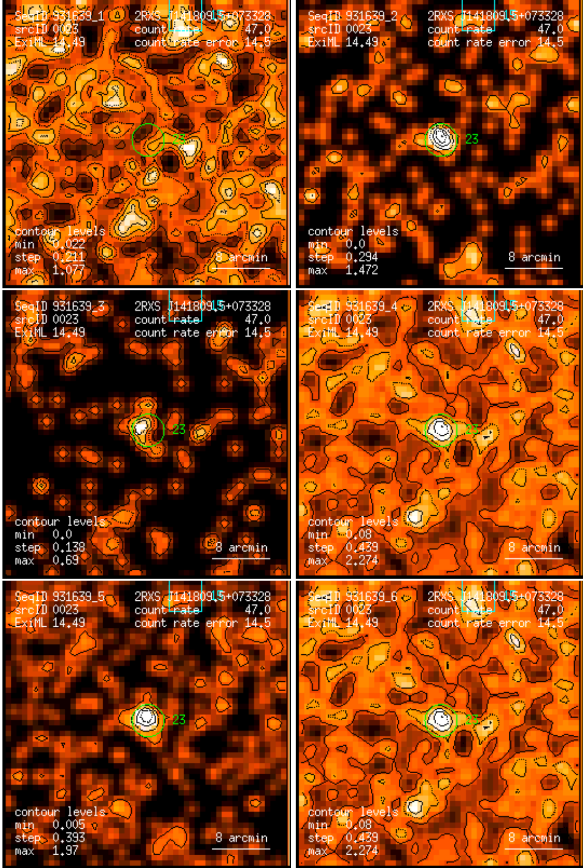
Figure 23: RASS 931639: detection 0023: band rate images, Gaussian filter: (1) PSPC channels 11 – 41, (2) 52 – 90, (3) 91 – 201, (4) 11 – 235, (5) 52 – 201, (6) 11 – 201. Broad band rates in counts/ks. Band rate contour levels in counts/ks/arcmin 2 .
