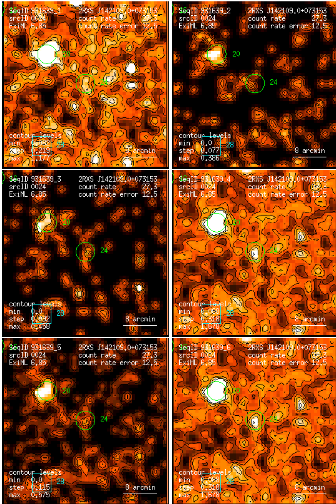
Figure 24: RASS 931639: detection 0024: band rate images, Gaussian filter: (1) PSPC channels 11 – 41, (2) 52 – 90, (3) 91 – 201, (4) 11 – 235, (5) 52 – 201, (6) 11 – 201. Broad band rates in counts/ks. Band rate contour levels in counts/ks/arcmin 2 .
