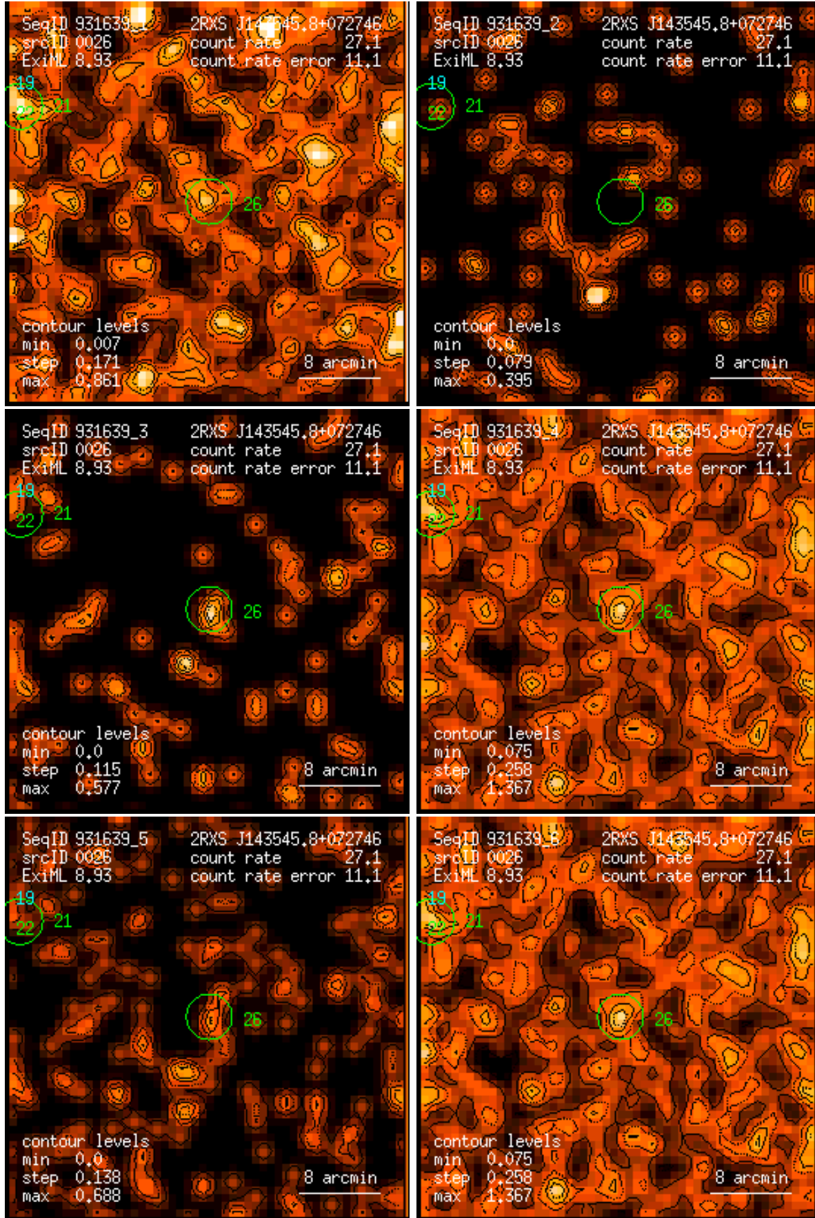
Figure 26: RASS 931639: detection 0026: band rate images, Gaussian filter: (1) PSPC channels 11 – 41, (2) 52 – 90, (3) 91 – 201, (4) 11 – 235, (5) 52 – 201, (6) 11 – 201. Broad band rates in counts/ks. Band rate contour levels in counts/ks/arcmin 2 .
