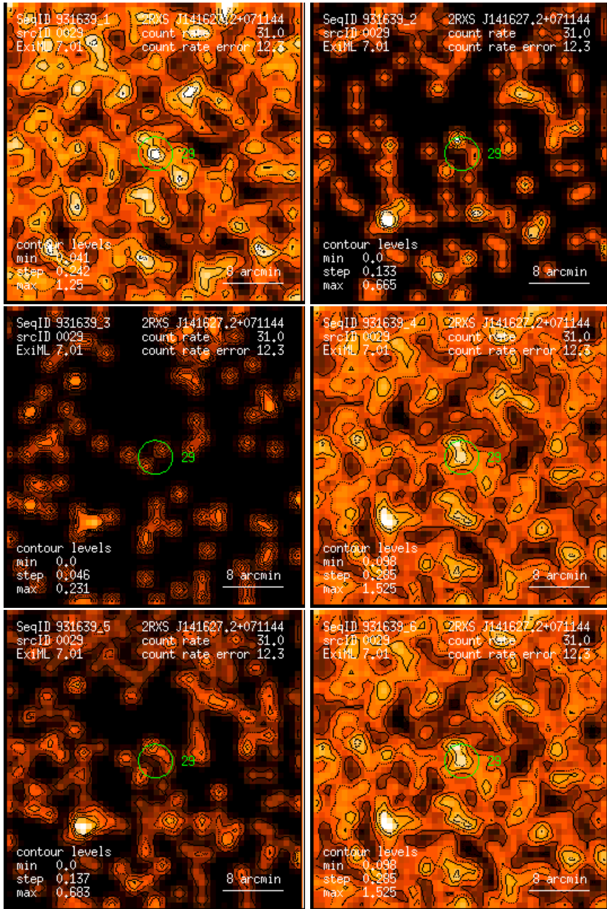
Figure 29: RASS 931639: detection 0029: band rate images, Gaussian filter: (1) PSPC channels 11 – 41, (2) 52 – 90, (3) 91 – 201, (4) 11 – 235, (5) 52 – 201, (6) 11 – 201. Broad band rates in counts/ks. Band rate contour levels in counts/ks/arcmin 2 .
