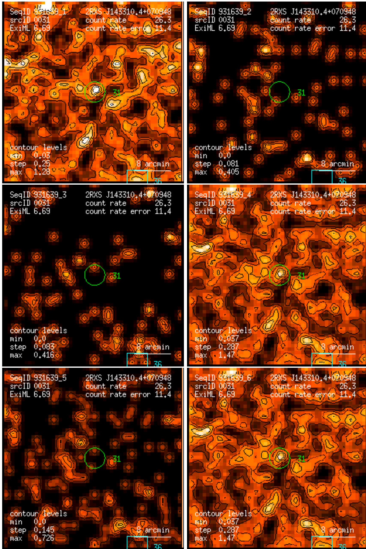
Figure 31: RASS 931639: detection 0031: band rate images, Gaussian filter: (1) PSPC channels 11 – 41, (2) 52 – 90, (3) 91 – 201, (4) 11 – 235, (5) 52 – 201, (6) 11 – 201. Broad band rates in counts/ks. Band rate contour levels in counts/ks/arcmin 2 .
