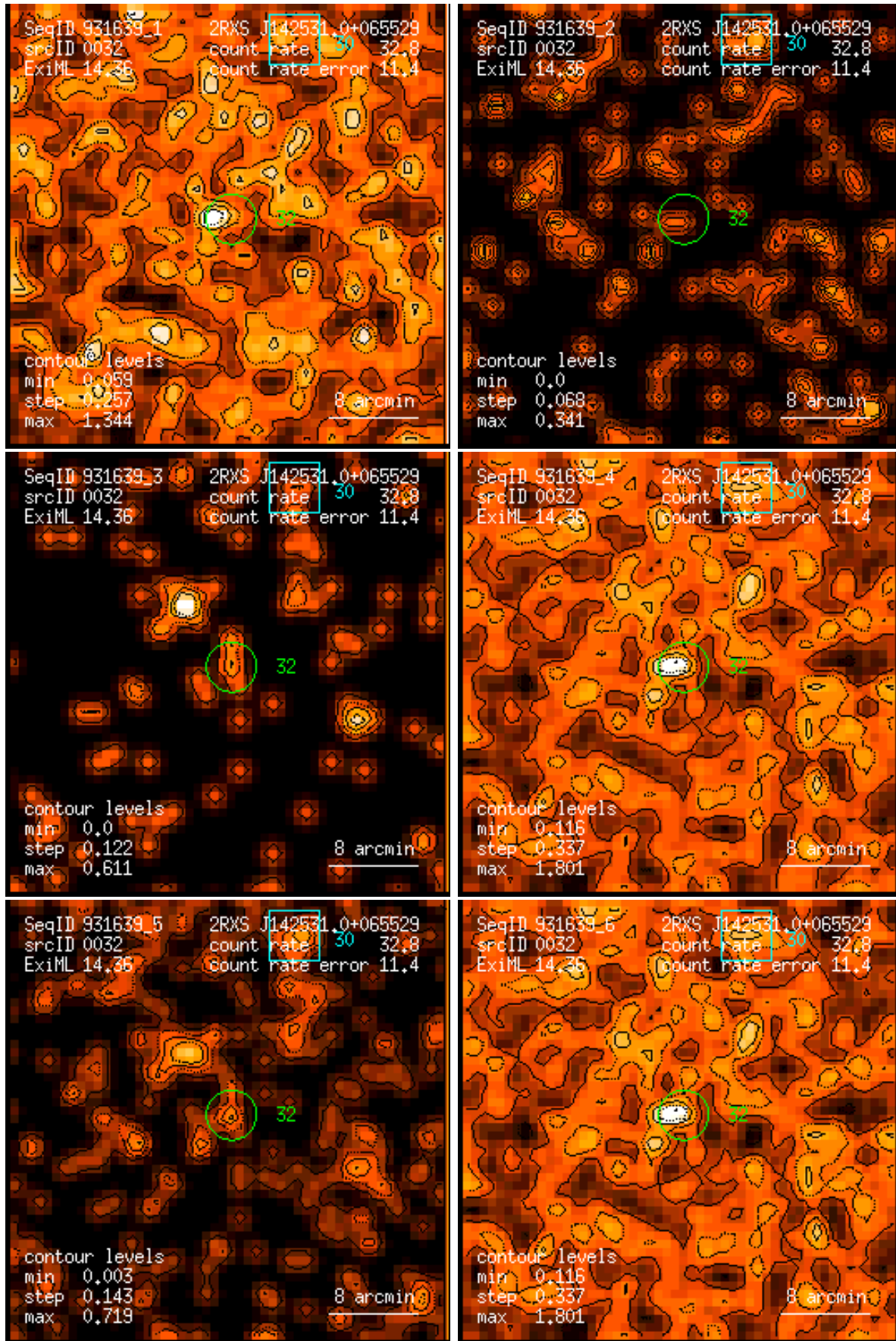
Figure 32: RASS 931639: detection 0032: band rate images, Gaussian filter: (1) PSPC channels 11 – 41, (2) 52 – 90, (3) 91 – 201, (4) 11 – 235, (5) 52 – 201, (6) 11 – 201. Broad band rates in counts/ks. Band rate contour levels in counts/ks/arcmin 2 .
