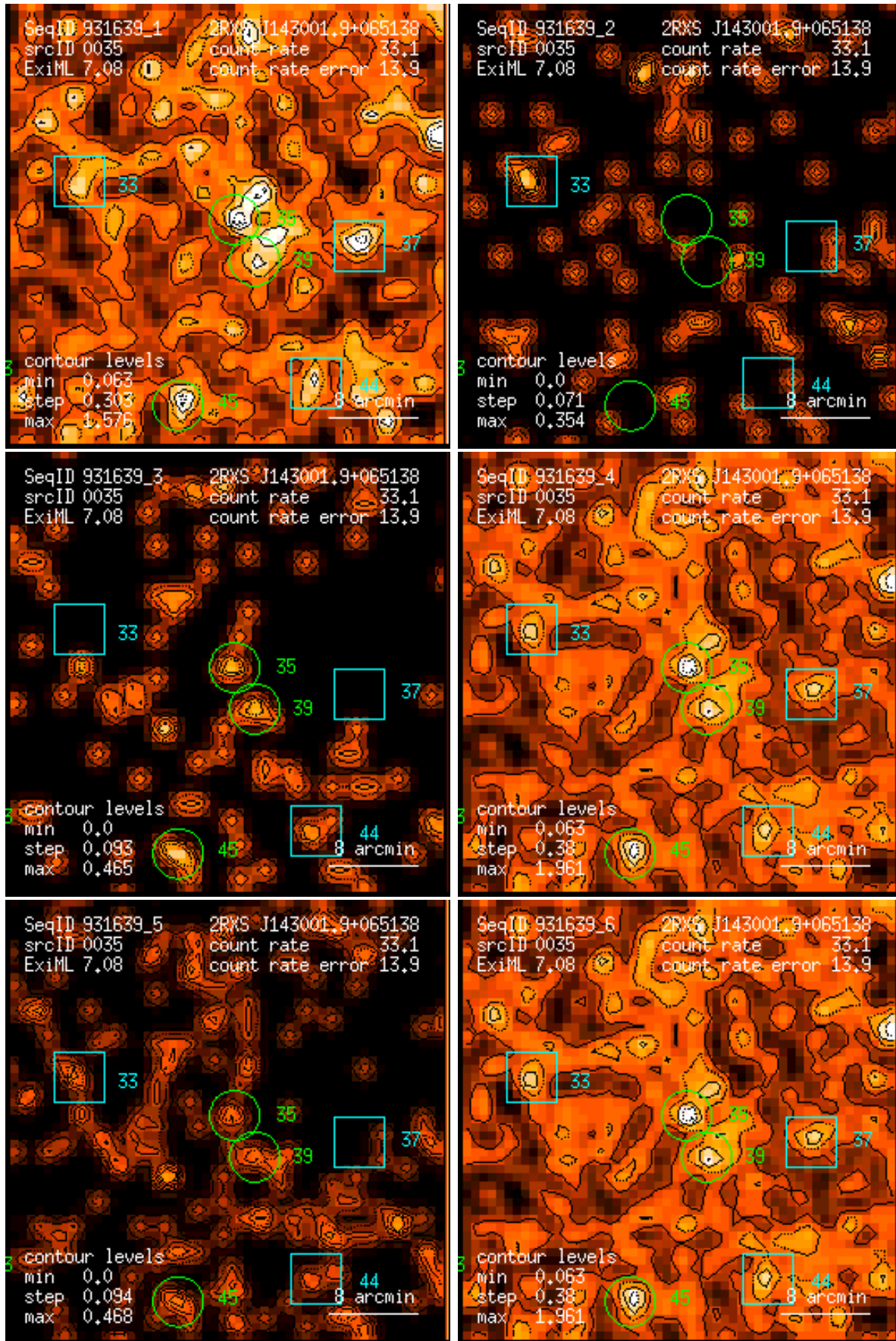
Figure 35: RASS 931639: detection 0035: band rate images, Gaussian filter: (1) PSPC channels 11 – 41, (2) 52 – 90, (3) 91 – 201, (4) 11 – 235, (5) 52 – 201, (6) 11 – 201. Broad band rates in counts/ks. Band rate contour levels in counts/ks/arcmin 2 .
