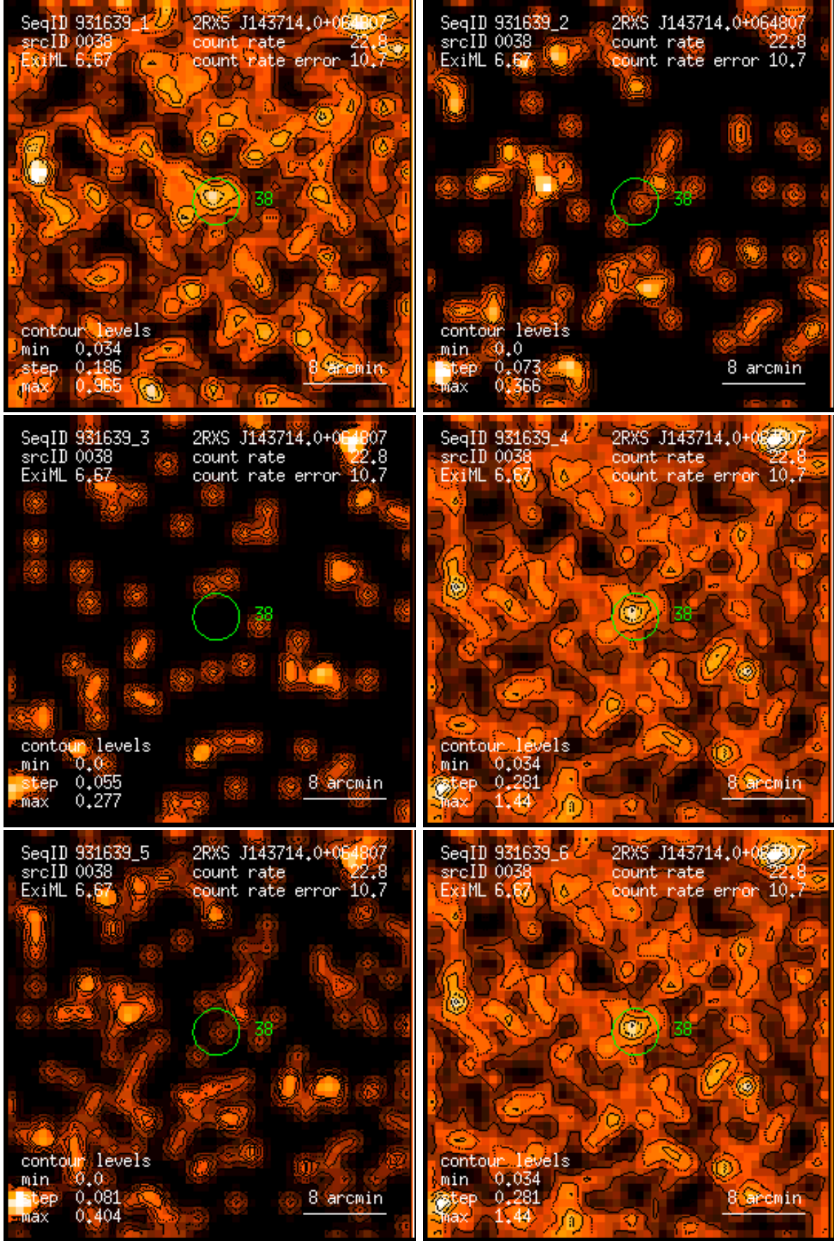
Figure 38: RASS 931639: detection 0038: band rate images, Gaussian filter: (1) PSPC channels 11 – 41, (2) 52 – 90, (3) 91 – 201, (4) 11 – 235, (5) 52 – 201, (6) 11 – 201. Broad band rates in counts/ks. Band rate contour levels in counts/ks/arcmin 2 .
