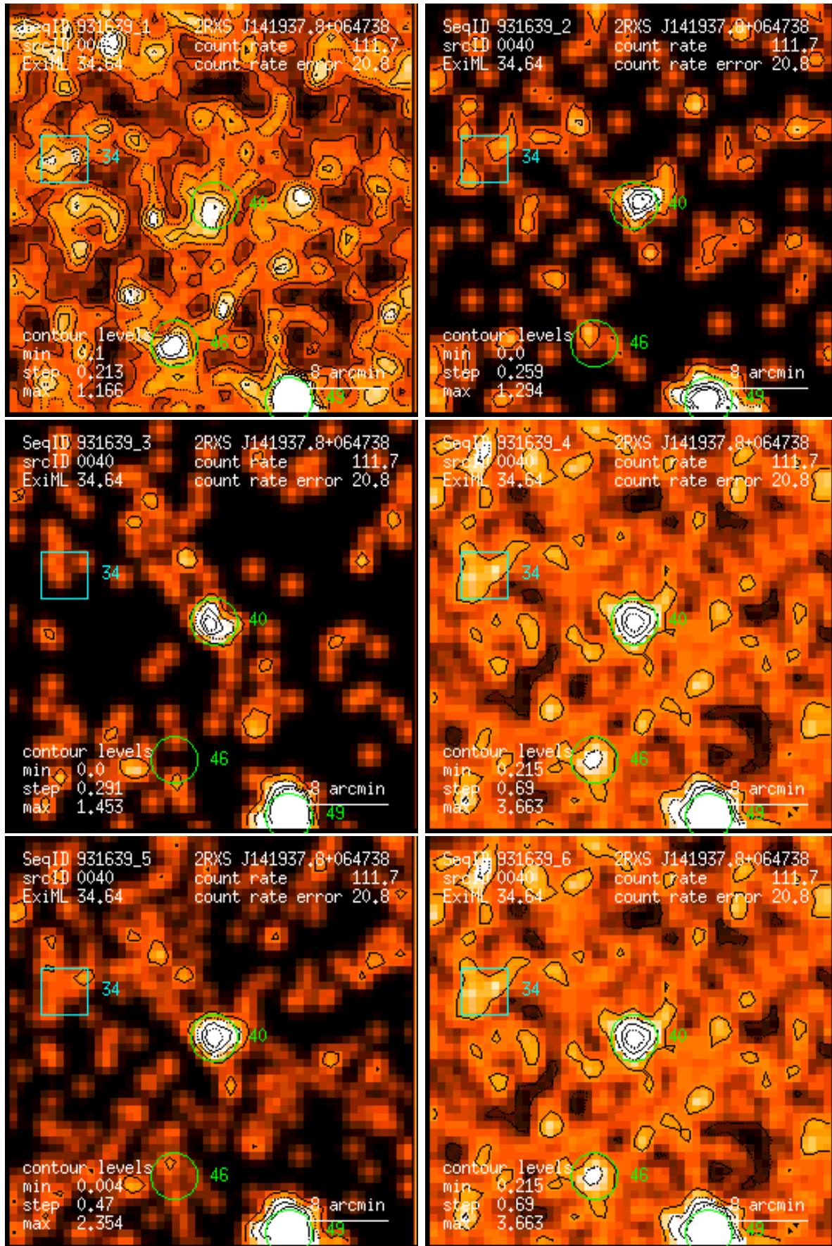
Figure 40: RASS 931639: detection 0040: band rate images, Gaussian filter: (1) PSPC channels 11 – 41, (2) 52 – 90, (3) 91 – 201, (4) 11 – 235, (5) 52 – 201, (6) 11 – 201. Broad band rates in counts/ks. Band rate contour levels in counts/ks/arcmin 2 .
