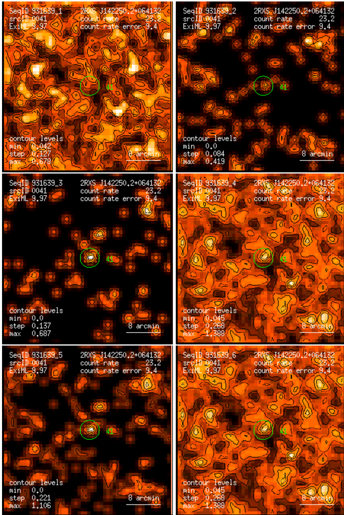
Figure 41: RASS 931639: detection 0041: band rate images, Gaussian filter: (1) PSPC channels 11 – 41, (2) 52 – 90, (3) 91 – 201, (4) 11 – 235, (5) 52 – 201, (6) 11 – 201. Broad band rates in counts/ks. Band rate contour levels in counts/ks/arcmin 2 .
