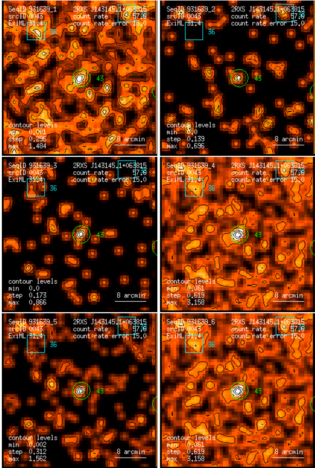
Figure 43: RASS 931639: detection 0043: band rate images, Gaussian filter: (1) PSPC channels 11 – 41, (2) 52 – 90, (3) 91 – 201, (4) 11 – 235, (5) 52 – 201, (6) 11 – 201. Broad band rates in counts/ks. Band rate contour levels in counts/ks/arcmin 2 .
