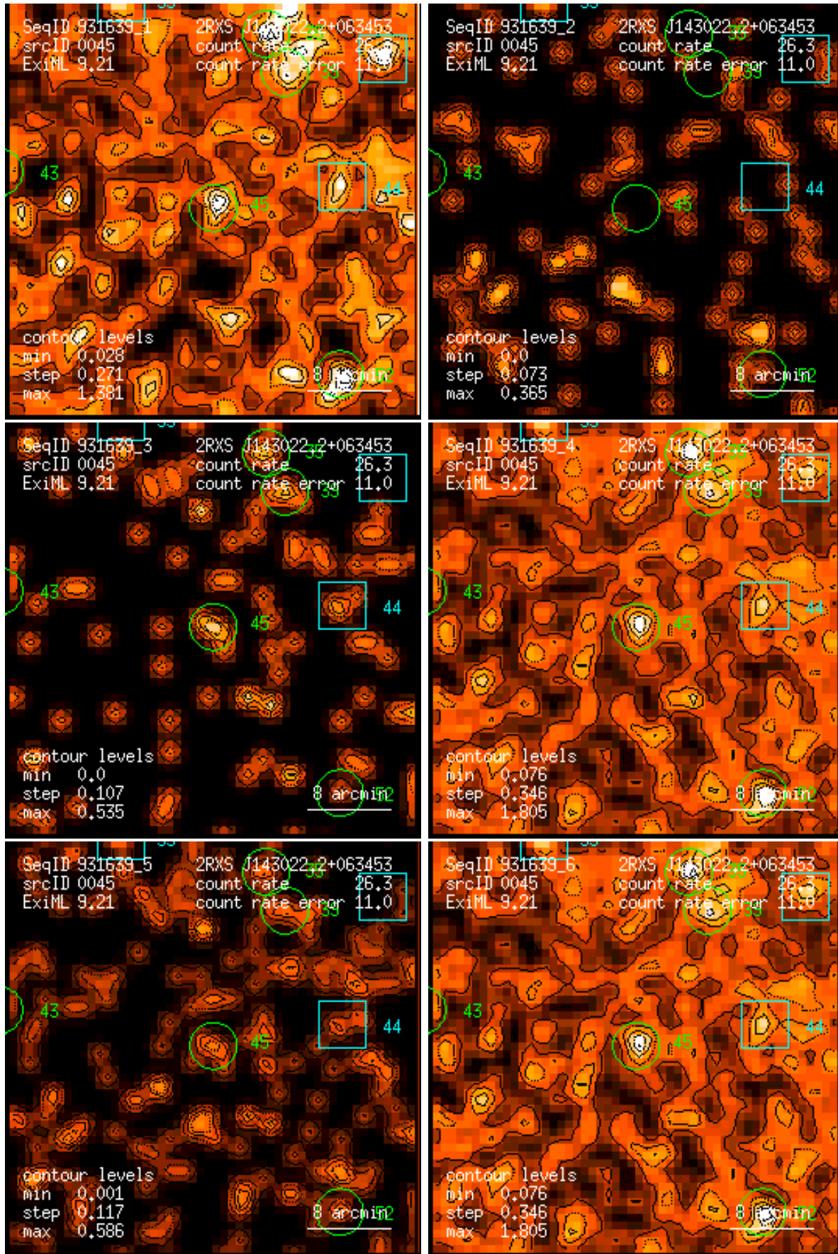
Figure 45: RASS 931639: detection 0045: band rate images, Gaussian filter: (1) PSPC channels 11 – 41, (2) 52 – 90, (3) 91 – 201, (4) 11 – 235, (5) 52 – 201, (6) 11 – 201. Broad band rates in counts/ks. Band rate contour levels in counts/ks/arcmin 2 .
